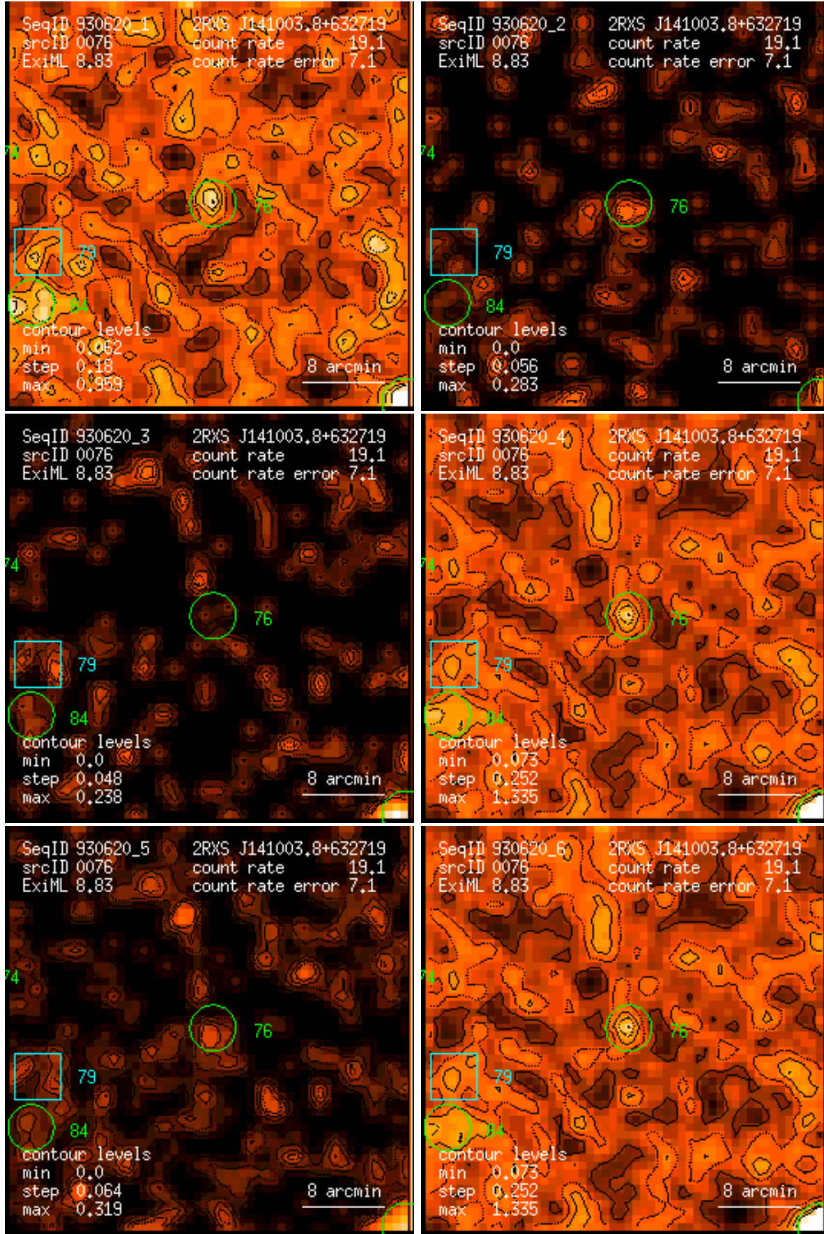
Figure 76: RASS 930620: detection 0076: band rate images, Gaussian filter: (1) PSPC channels 11 – 41, (2) 52 – 90, (3) 91 – 201, (4) 11 – 235, (5) 52 – 201, (6) 11 – 201. Broad band rates in counts/ks. Band rate contour levels in counts/ks/arcmin 2 .
