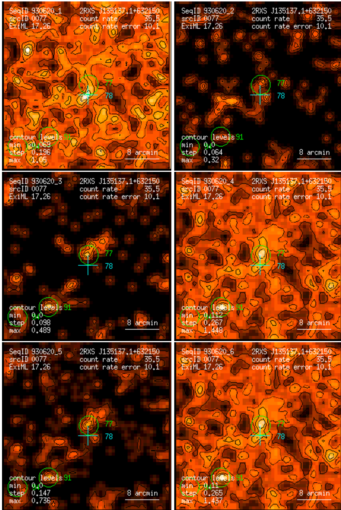
Figure 77: RASS 930620: detection 0077: band rate images, Gaussian filter: (1) PSPC channels 11 – 41, (2) 52 – 90, (3) 91 – 201, (4) 11 – 235, (5) 52 – 201, (6) 11 – 201. Broad band rates in counts/ks. Band rate contour levels in counts/ks/arcmin 2 .
