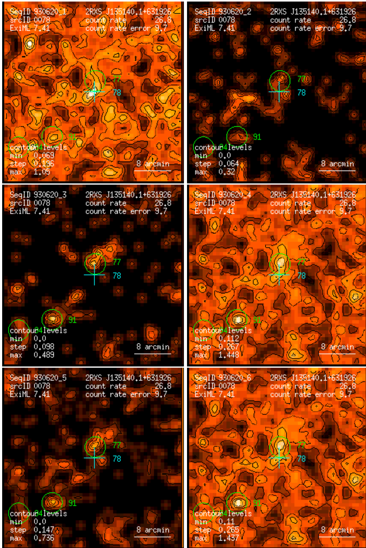
Figure 78: RASS 930620: detection 0078: band rate images, Gaussian filter: (1) PSPC channels 11 – 41, (2) 52 – 90, (3) 91 – 201, (4) 11 – 235, (5) 52 – 201, (6) 11 – 201. Broad band rates in counts/ks. Band rate contour levels in counts/ks/arcmin 2 .
