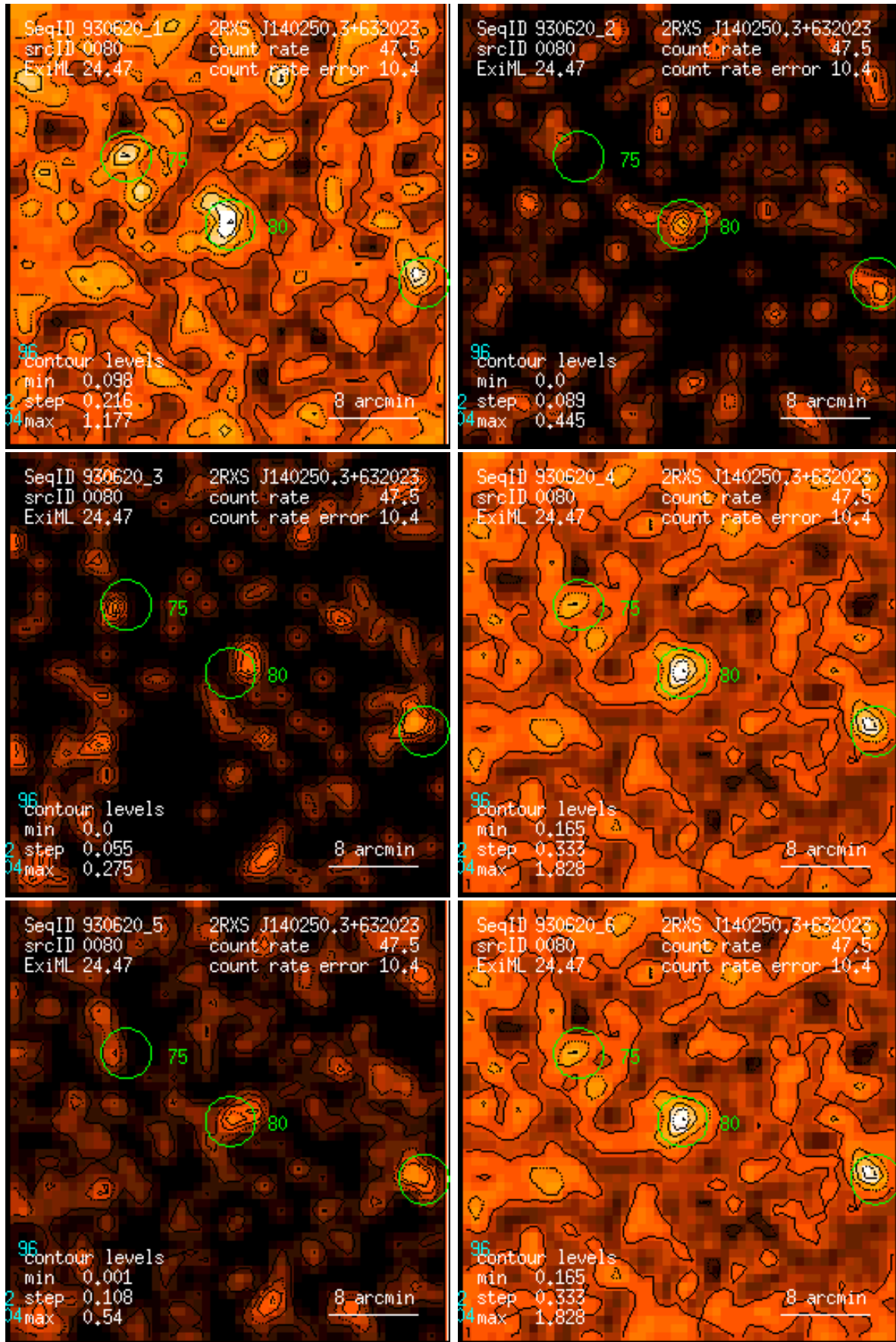
Figure 80: RASS 930620: detection 0080: band rate images, Gaussian filter: (1) PSPC channels 11 – 41, (2) 52 – 90, (3) 91 – 201, (4) 11 – 235, (5) 52 – 201, (6) 11 – 201. Broad band rates in counts/ks. Band rate contour levels in counts/ks/arcmin 2 .
