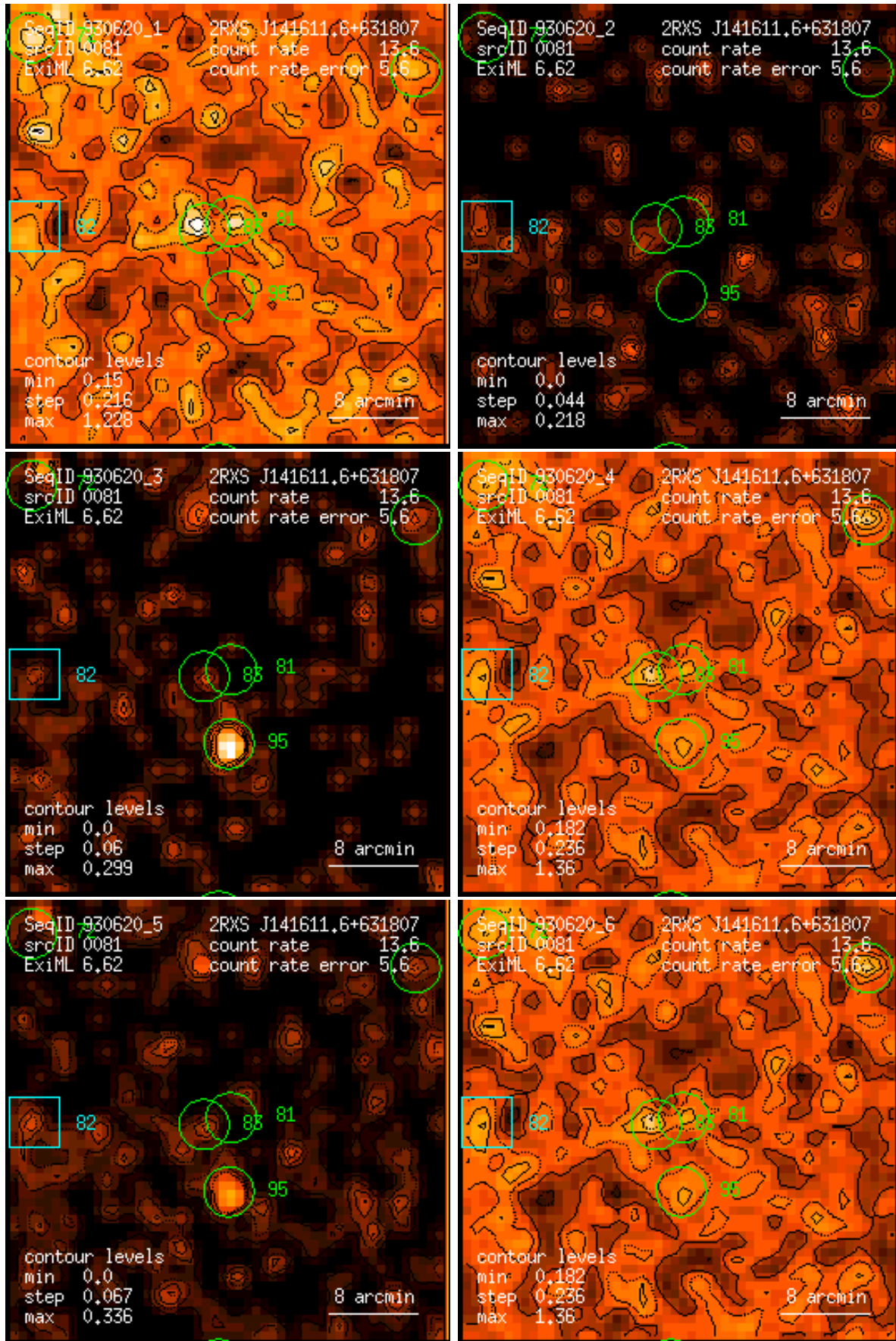
Figure 81: RASS 930620: detection 0081: band rate images, Gaussian filter: (1) PSPC channels 11 – 41, (2) 52 – 90, (3) 91 – 201, (4) 11 – 235, (5) 52 – 201, (6) 11 – 201. Broad band rates in counts/ks. Band rate contour levels in counts/ks/arcmin 2 .
