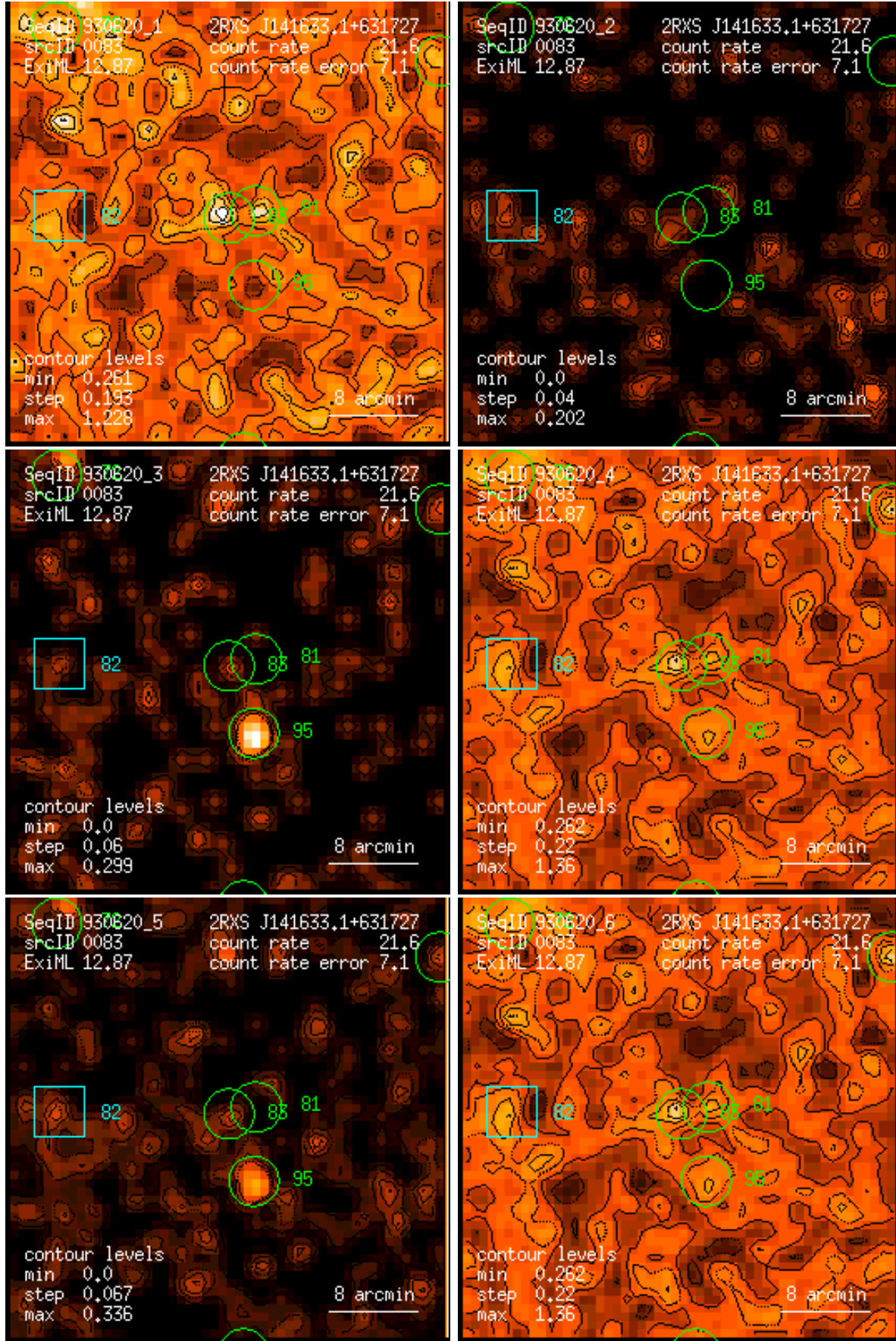
Figure 83: RASS 930620: detection 0083: band rate images, Gaussian filter: (1) PSPC channels 11 – 41, (2) 52 – 90, (3) 91 – 201, (4) 11 – 235, (5) 52 – 201, (6) 11 – 201. Broad band rates in counts/ks. Band rate contour levels in counts/ks/arcmin 2 .
