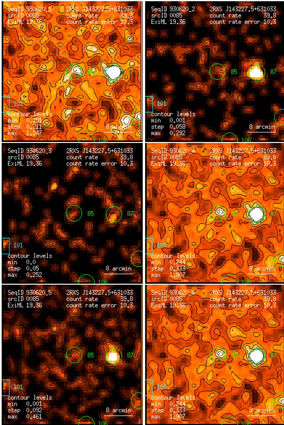
Figure 85: RASS 930620: detection 0085: band rate images, Gaussian filter: (1) PSPC channels 11 – 41, (2) 52 – 90, (3) 91 – 201, (4) 11 – 235, (5) 52 – 201, (6) 11 – 201. Broad band rates in counts/ks. Band rate contour levels in counts/ks/arcmin 2 .
