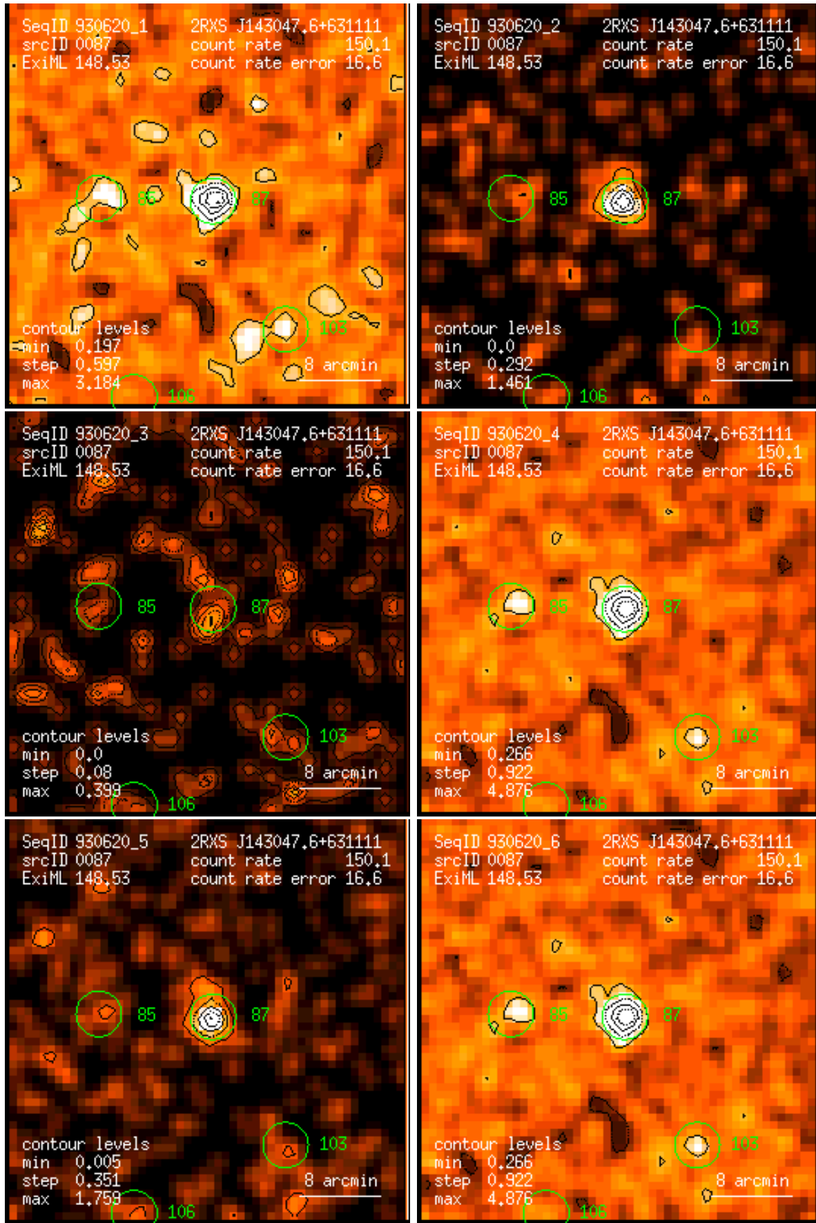
Figure 87: RASS 930620: detection 0087: band rate images, Gaussian filter: (1) PSPC channels 11 – 41, (2) 52 – 90, (3) 91 – 201, (4) 11 – 235, (5) 52 – 201, (6) 11 – 201. Broad band rates in counts/ks. Band rate contour levels in counts/ks/arcmin 2 .
