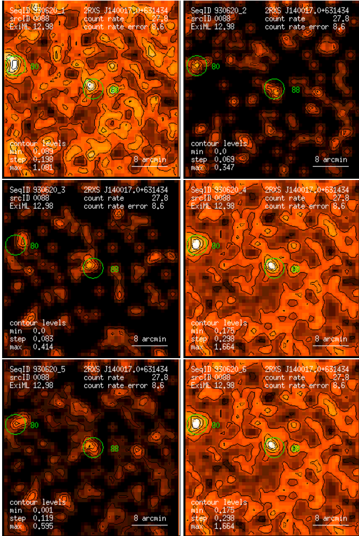
Figure 88: RASS 930620: detection 0088: band rate images, Gaussian filter: (1) PSPC channels 11 – 41, (2) 52 – 90, (3) 91 – 201, (4) 11 – 235, (5) 52 – 201, (6) 11 – 201. Broad band rates in counts/ks. Band rate contour levels in counts/ks/arcmin 2 .
