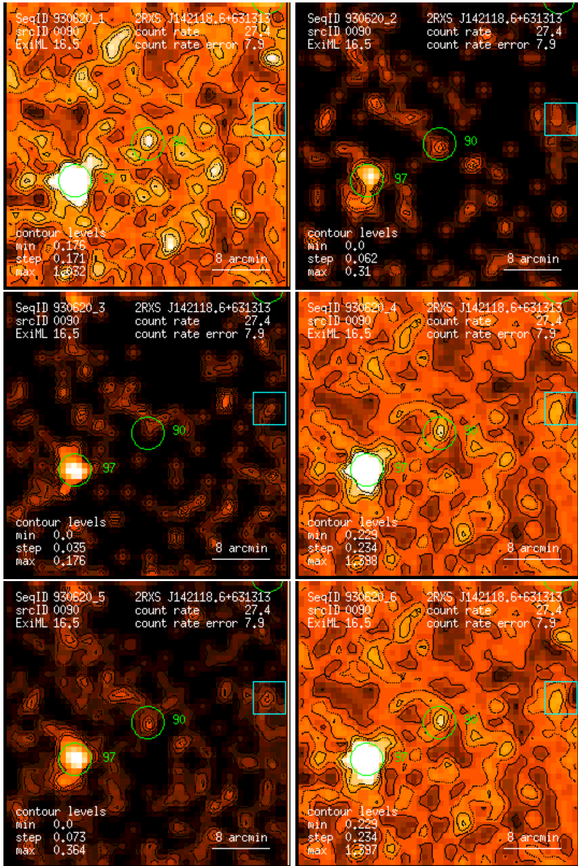
Figure 90: RASS 930620: detection 0090: band rate images, Gaussian filter: (1) PSPC channels 11 – 41, (2) 52 – 90, (3) 91 – 201, (4) 11 – 235, (5) 52 – 201, (6) 11 – 201. Broad band rates in counts/ks. Band rate contour levels in counts/ks/arcmin 2 .
