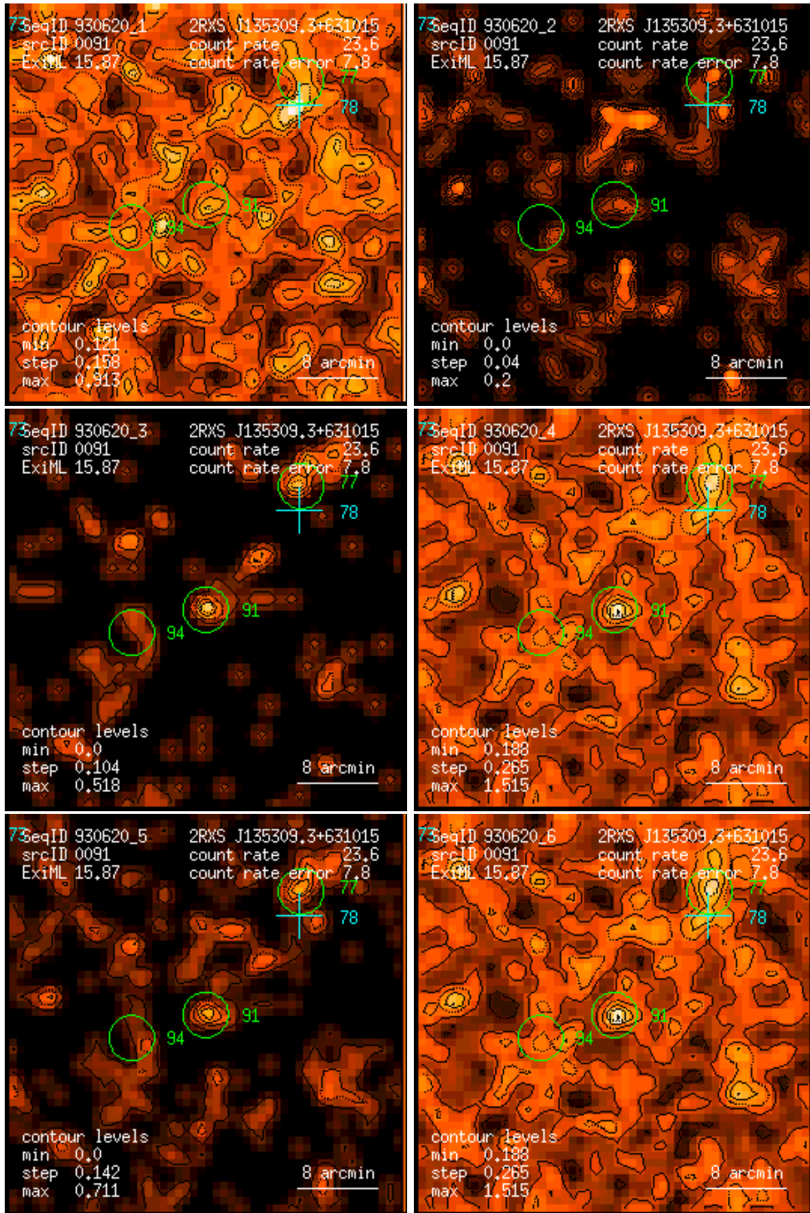
Figure 91: RASS 930620: detection 0091: band rate images, Gaussian filter: (1) PSPC channels 11 – 41, (2) 52 – 90, (3) 91 – 201, (4) 11 – 235, (5) 52 – 201, (6) 11 – 201. Broad band rates in counts/ks. Band rate contour levels in counts/ks/arcmin 2 .
