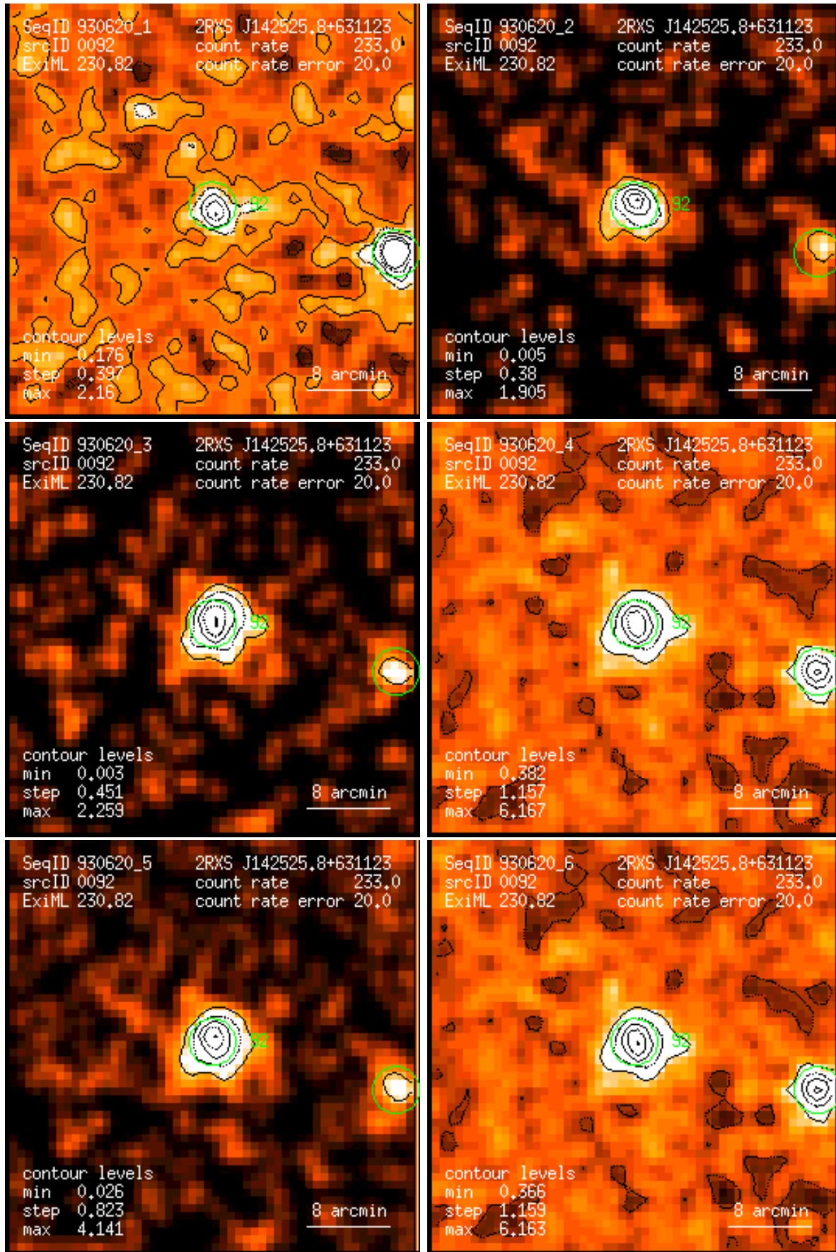
Figure 92: RASS 930620: detection 0092: band rate images, Gaussian filter: (1) PSPC channels 11 – 41, (2) 52 – 90, (3) 91 – 201, (4) 11 – 235, (5) 52 – 201, (6) 11 – 201. Broad band rates in counts/ks. Band rate contour levels in counts/ks/arcmin 2 .
