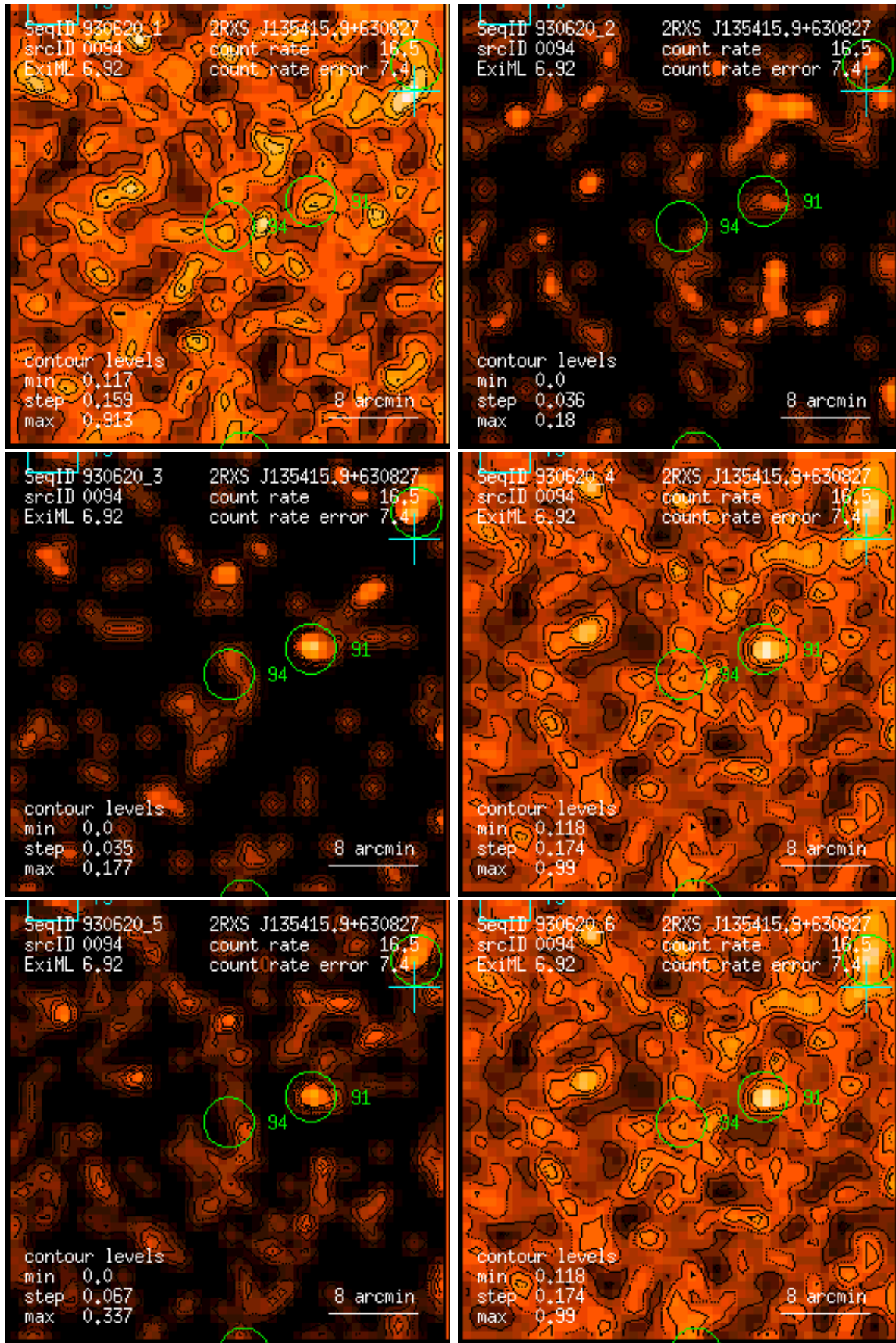
Figure 94: RASS 930620: detection 0094: band rate images, Gaussian filter: (1) PSPC channels 11 – 41, (2) 52 – 90, (3) 91 – 201, (4) 11 – 235, (5) 52 – 201, (6) 11 – 201. Broad band rates in counts/ks. Band rate contour levels in counts/ks/arcmin 2 .
