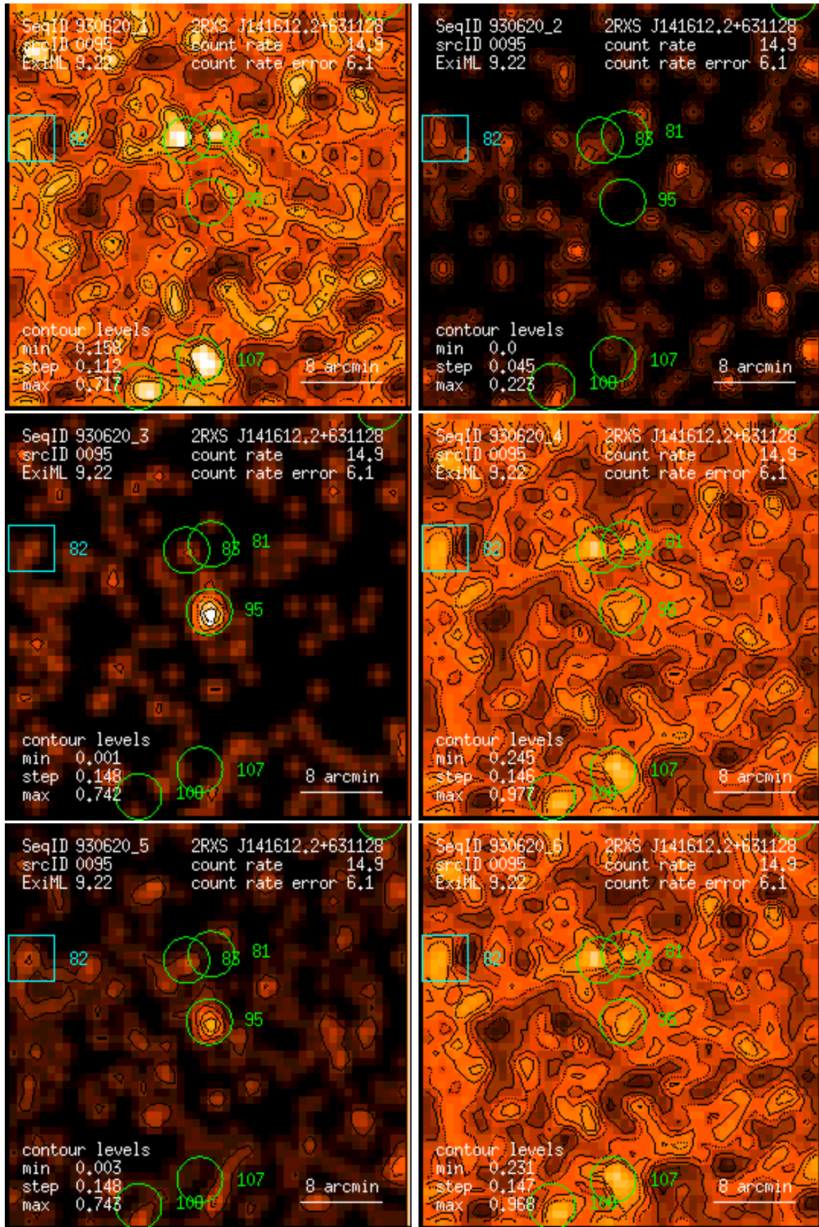
Figure 95: RASS 930620: detection 0095: band rate images, Gaussian filter: (1) PSPC channels 11 – 41, (2) 52 – 90, (3) 91 – 201, (4) 11 – 235, (5) 52 – 201, (6) 11 – 201. Broad band rates in counts/ks. Band rate contour levels in counts/ks/arcmin 2 .
