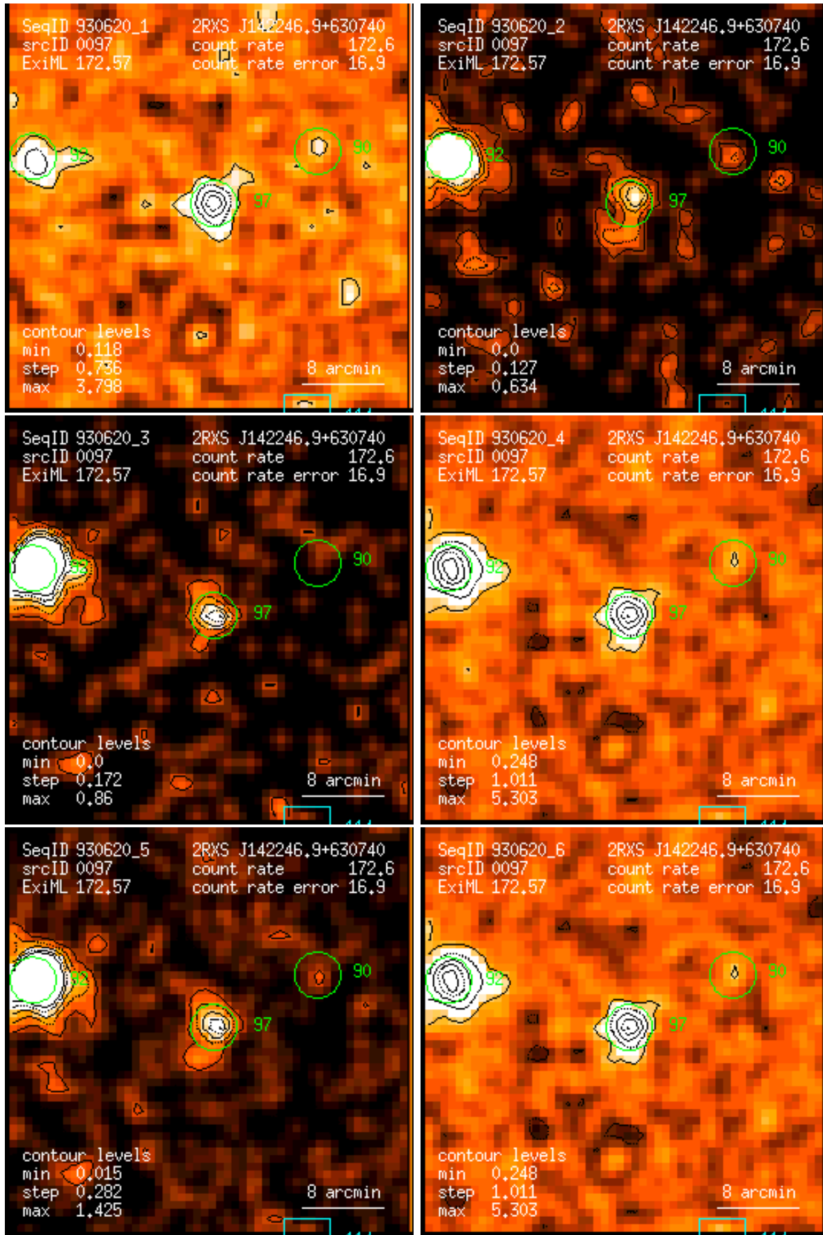
Figure 97: RASS 930620: detection 0097: band rate images, Gaussian filter: (1) PSPC channels 11 – 41, (2) 52 – 90, (3) 91 – 201, (4) 11 – 235, (5) 52 – 201, (6) 11 – 201. Broad band rates in counts/ks. Band rate contour levels in counts/ks/arcmin 2 .
