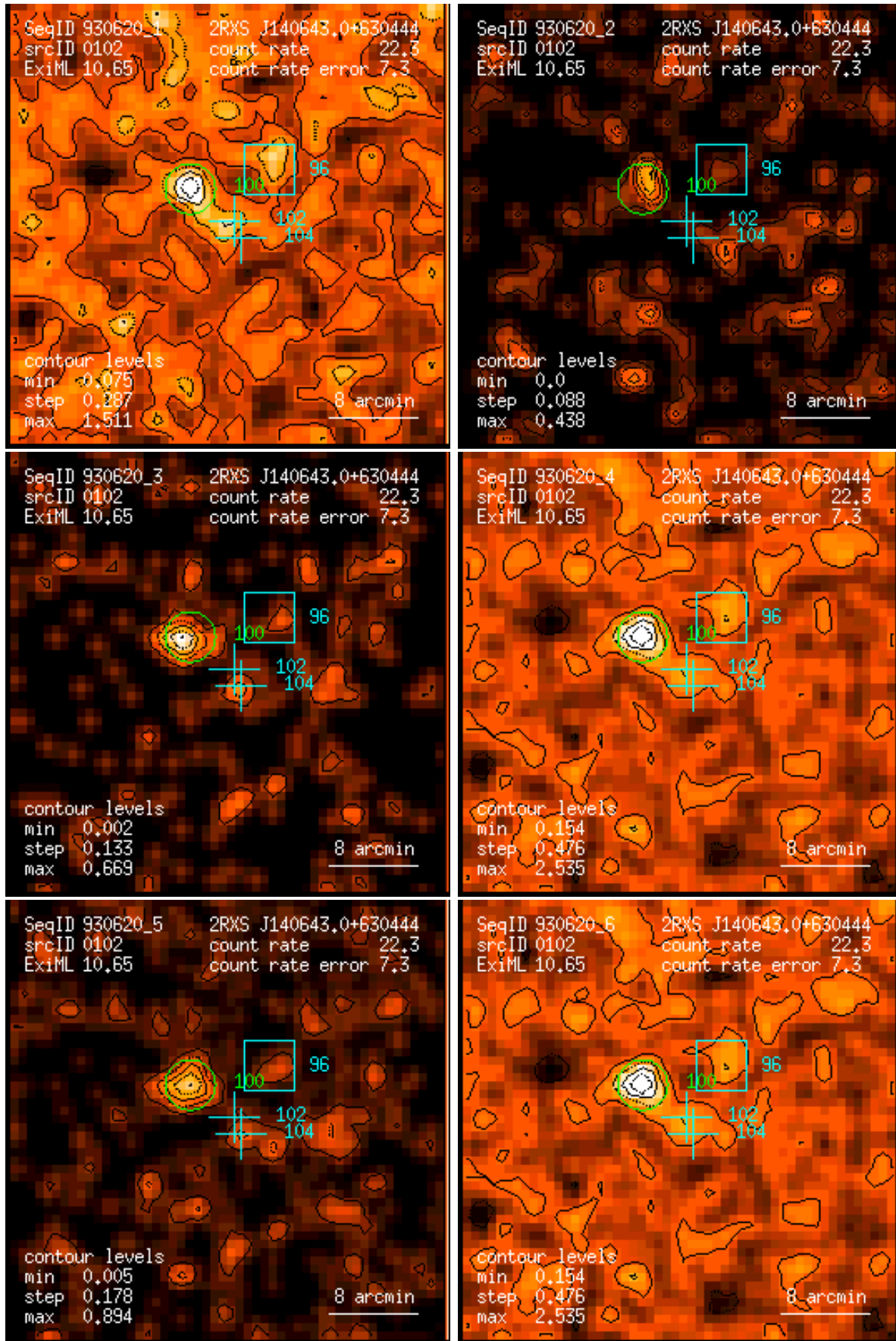
Figure 102: RASS 930620: detection 0102: band rate images, Gaussian filter: (1) PSPC channels 11 – 41, (2) 52 – 90, (3) 91 – 201, (4) 11 – 235, (5) 52 – 201, (6) 11 – 201. Broad band rates in counts/ks. Band rate contour levels in counts/ks/arcmin 2 .
