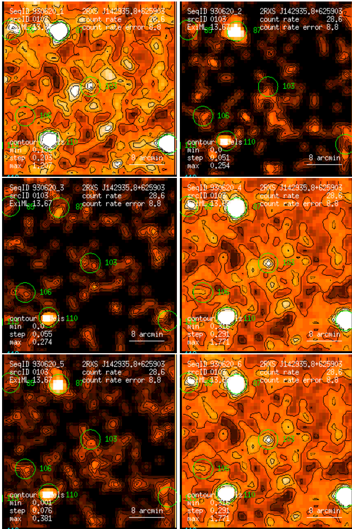
Figure 103: RASS 930620: detection 0103: band rate images, Gaussian filter: (1) PSPC channels 11 – 41, (2) 52 – 90, (3) 91 – 201, (4) 11 – 235, (5) 52 – 201, (6) 11 – 201. Broad band rates in counts/ks. Band rate contour levels in counts/ks/arcmin 2 .
