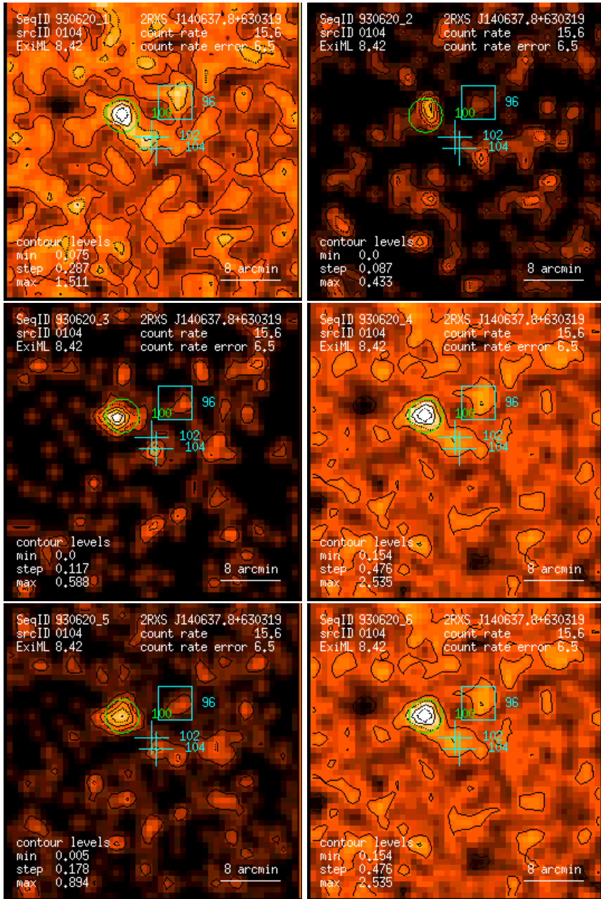
Figure 104: RASS 930620: detection 0104: band rate images, Gaussian filter: (1) PSPC channels 11 – 41, (2) 52 – 90, (3) 91 – 201, (4) 11 – 235, (5) 52 – 201, (6) 11 – 201. Broad band rates in counts/ks. Band rate contour levels in counts/ks/arcmin 2 .
