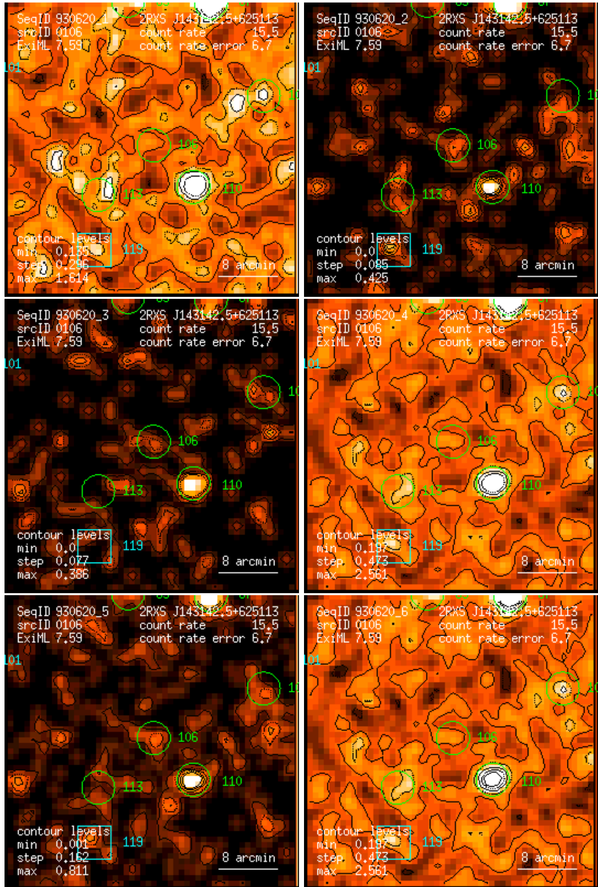
Figure 106: RASS 930620: detection 0106: band rate images, Gaussian filter: (1) PSPC channels 11 – 41, (2) 52 – 90, (3) 91 – 201, (4) 11 – 235, (5) 52 – 201, (6) 11 – 201. Broad band rates in counts/ks. Band rate contour levels in counts/ks/arcmin 2 .
