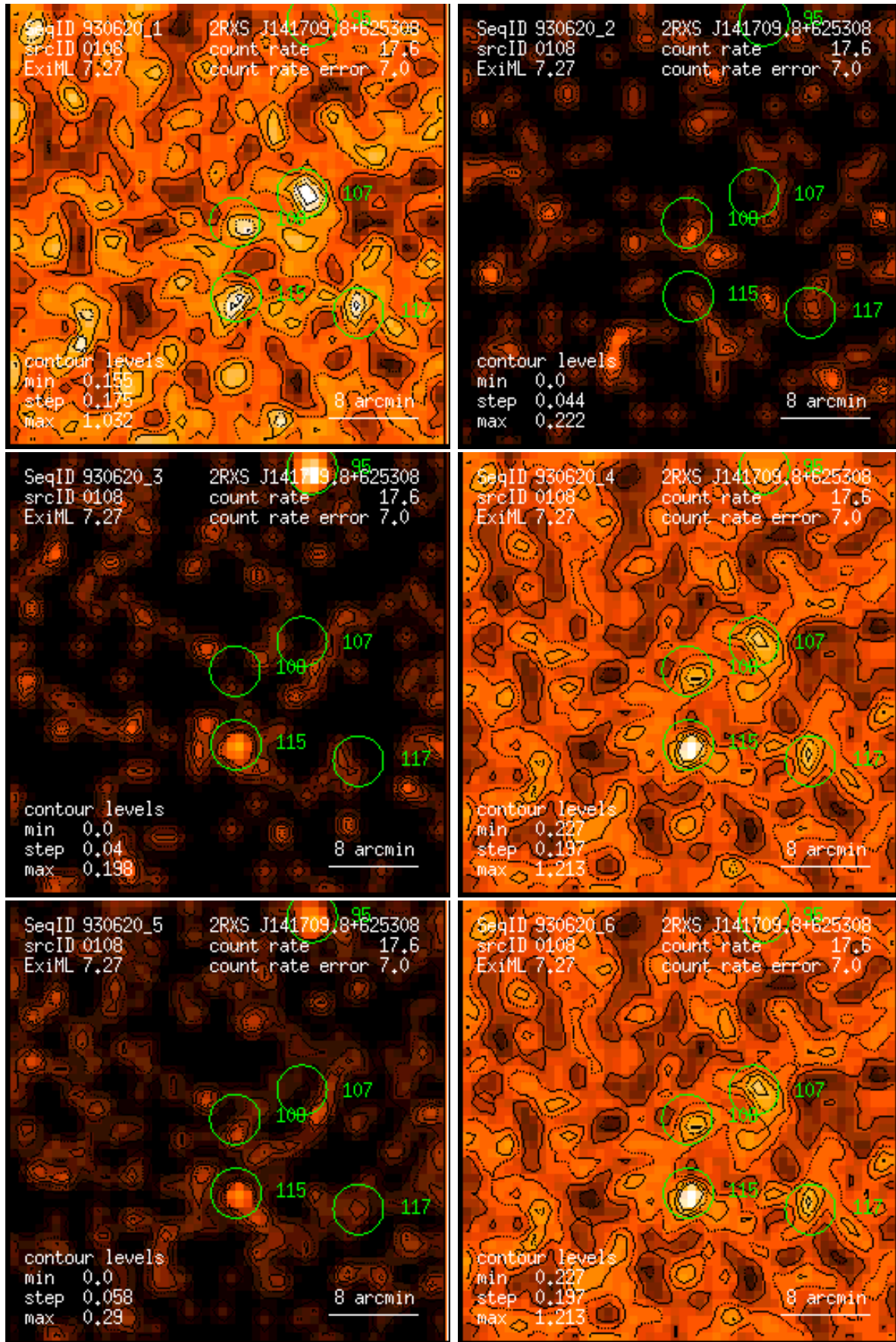
Figure 108: RASS 930620: detection 0108: band rate images, Gaussian filter: (1) PSPC channels 11 – 41, (2) 52 – 90, (3) 91 – 201, (4) 11 – 235, (5) 52 – 201, (6) 11 – 201. Broad band rates in counts/ks. Band rate contour levels in counts/ks/arcmin 2 .
