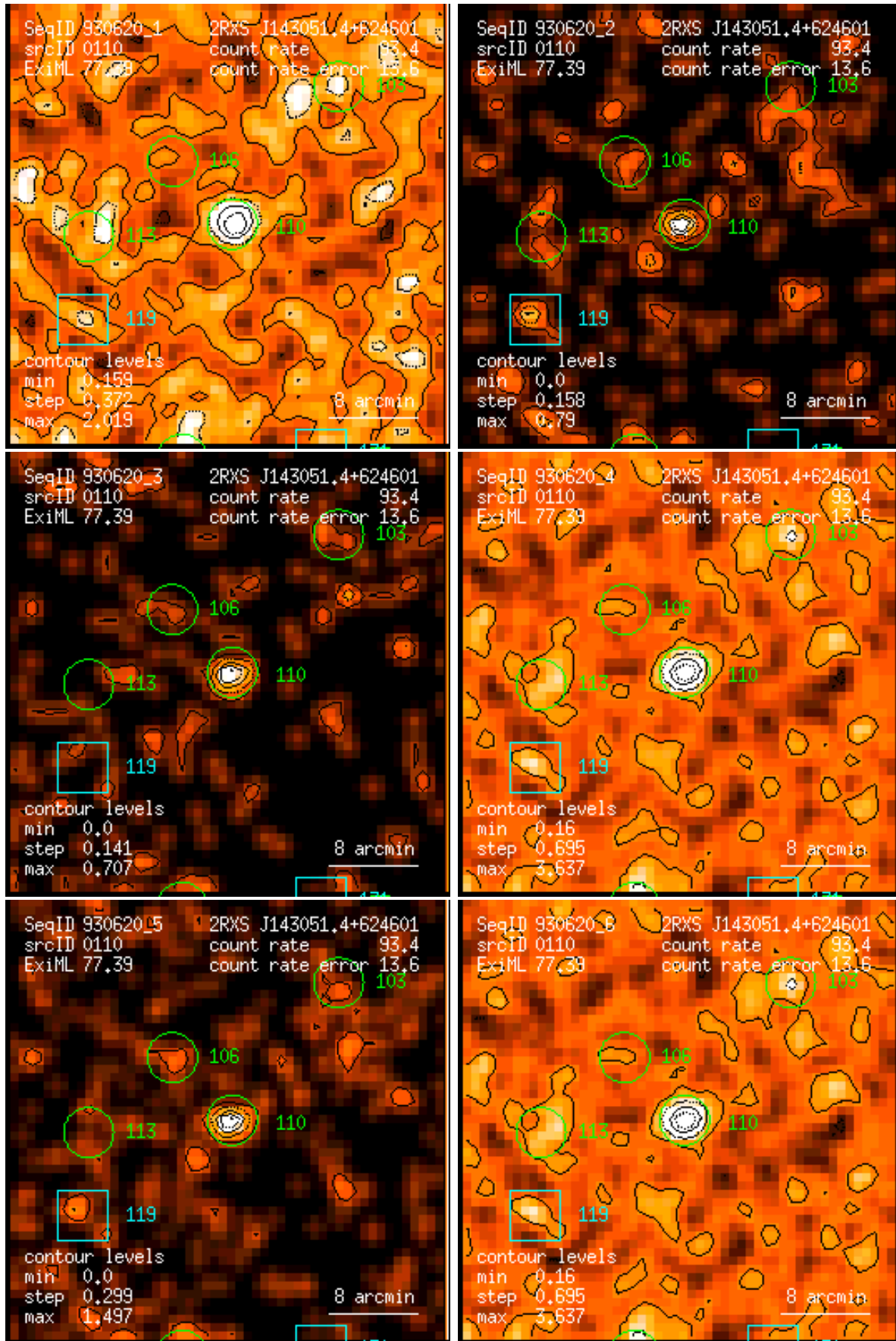
Figure 110: RASS 930620: detection 0110: band rate images, Gaussian filter: (1) PSPC channels 11 – 41, (2) 52 – 90, (3) 91 – 201, (4) 11 – 235, (5) 52 – 201, (6) 11 – 201. Broad band rates in counts/ks. Band rate contour levels in counts/ks/arcmin 2 .
