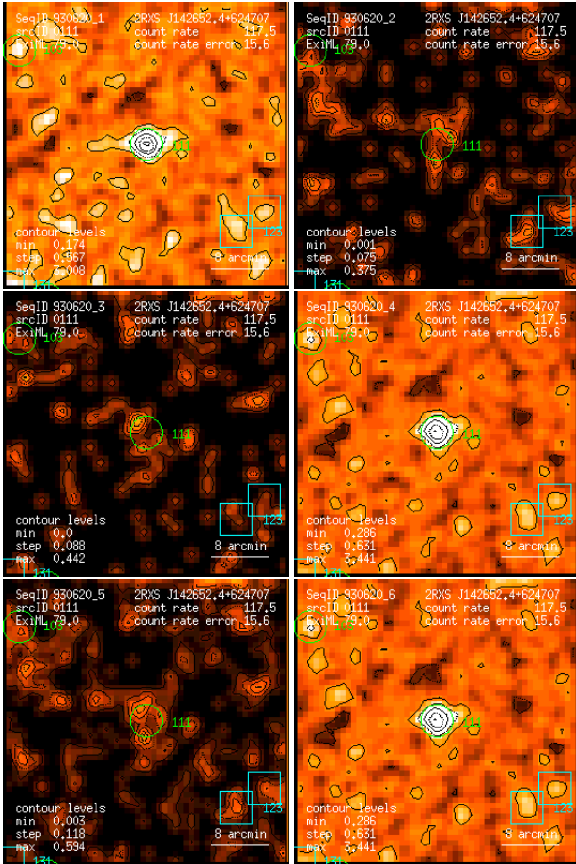
Figure 111: RASS 930620: detection 0111: band rate images, Gaussian filter: (1) PSPC channels 11 – 41, (2) 52 – 90, (3) 91 – 201, (4) 11 – 235, (5) 52 – 201, (6) 11 – 201. Broad band rates in counts/ks. Band rate contour levels in counts/ks/arcmin 2 .
