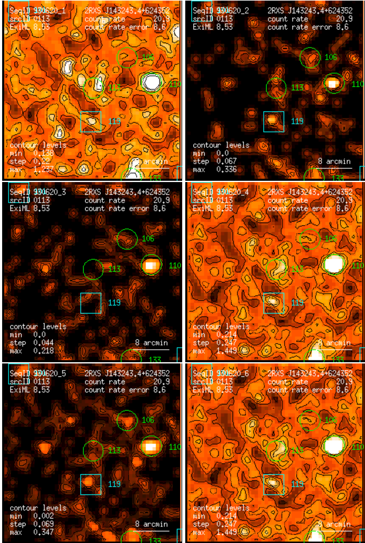
Figure 113: RASS 930620: detection 0113: band rate images, Gaussian filter: (1) PSPC channels 11 – 41, (2) 52 – 90, (3) 91 – 201, (4) 11 – 235, (5) 52 – 201, (6) 11 – 201. Broad band rates in counts/ks. Band rate contour levels in counts/ks/arcmin 2 .
