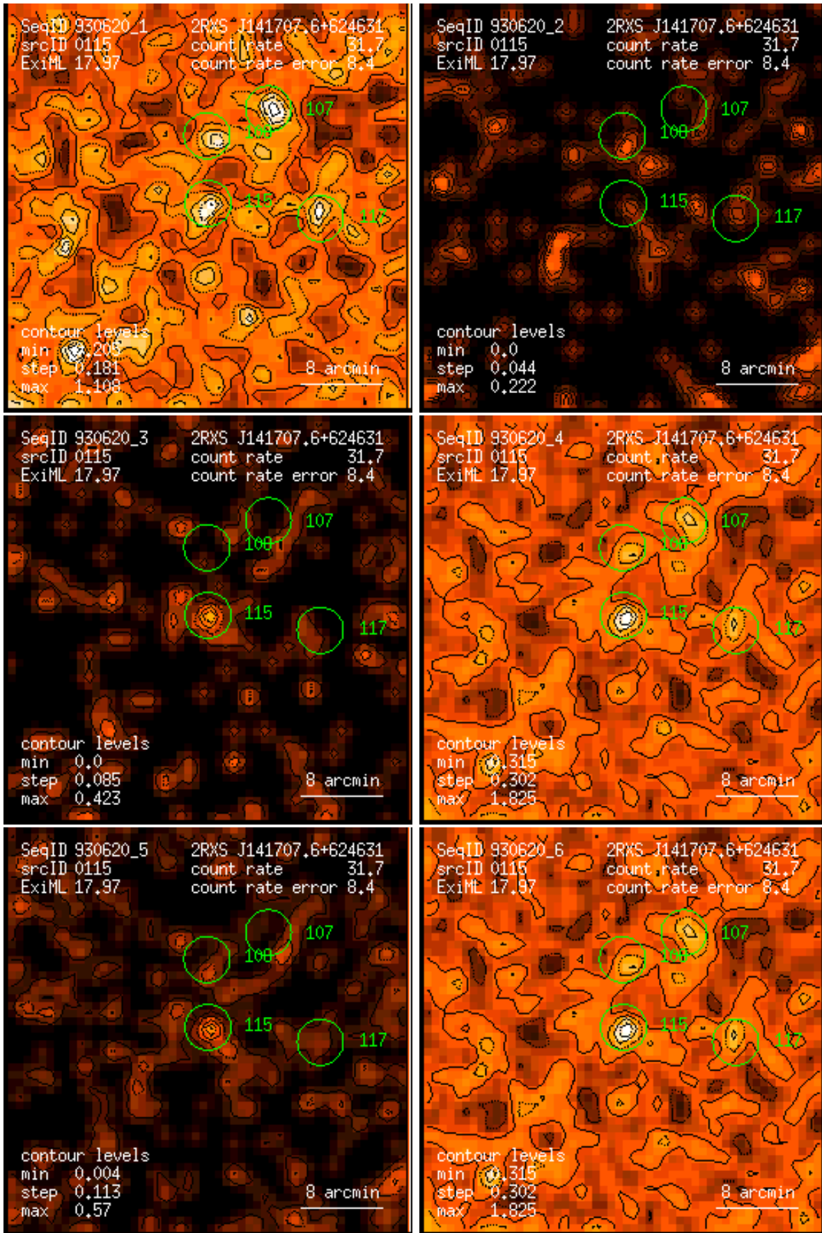
Figure 115: RASS 930620: detection 0115: band rate images, Gaussian filter: (1) PSPC channels 11 – 41, (2) 52 – 90, (3) 91 – 201, (4) 11 – 235, (5) 52 – 201, (6) 11 – 201. Broad band rates in counts/ks. Band rate contour levels in counts/ks/arcmin 2 .
