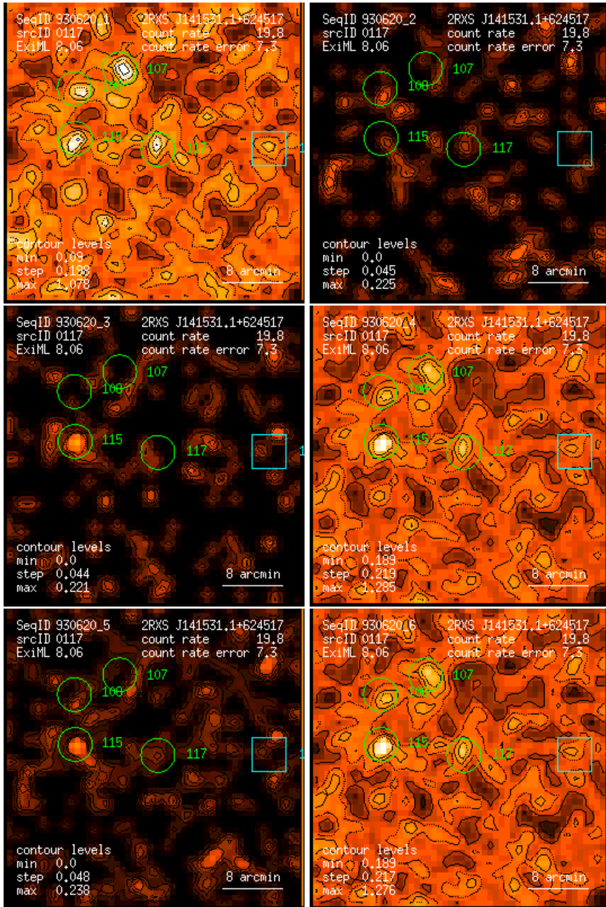
Figure 117: RASS 930620: detection 0117: band rate images, Gaussian filter: (1) PSPC channels 11 – 41, (2) 52 – 90, (3) 91 – 201, (4) 11 – 235, (5) 52 – 201, (6) 11 – 201. Broad band rates in counts/ks. Band rate contour levels in counts/ks/arcmin 2 .
