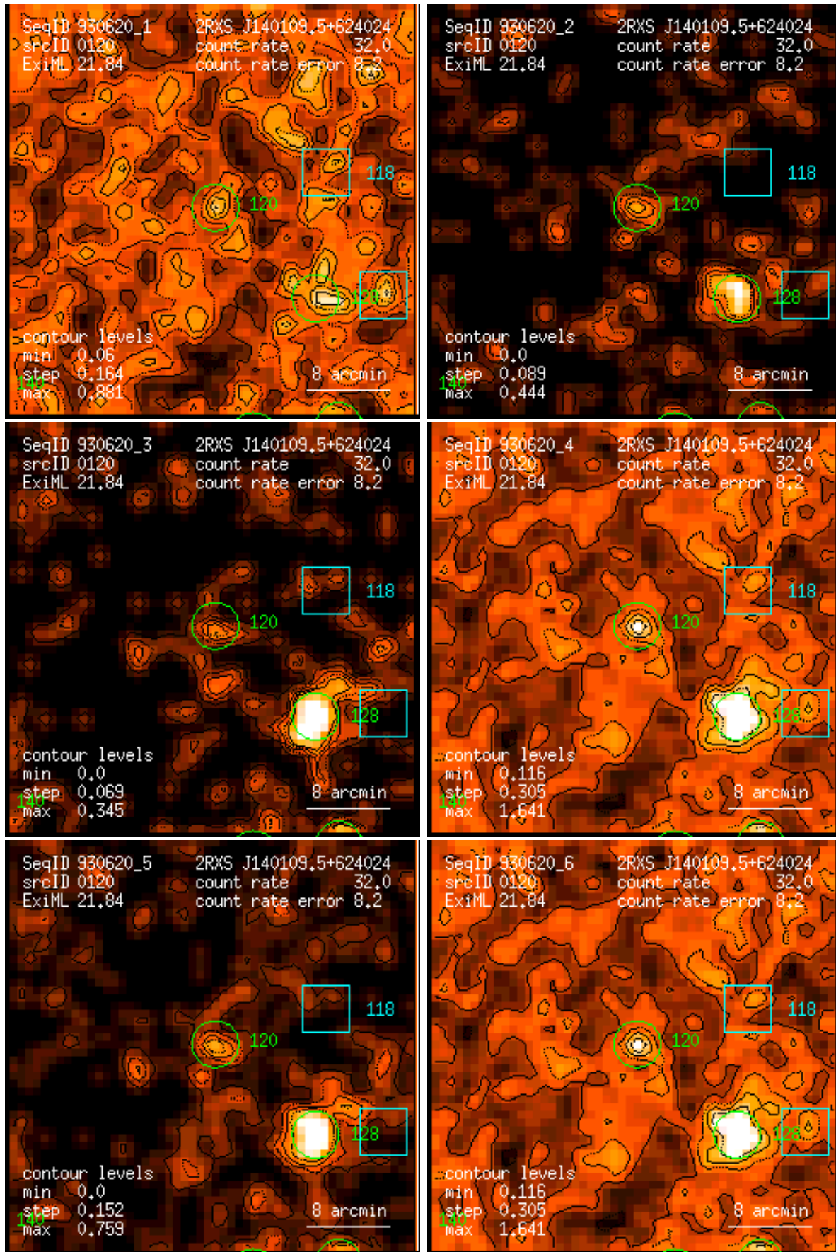
Figure 120: RASS 930620: detection 0120: band rate images, Gaussian filter: (1) PSPC channels 11 – 41, (2) 52 – 90, (3) 91 – 201, (4) 11 – 235, (5) 52 – 201, (6) 11 – 201. Broad band rates in counts/ks. Band rate contour levels in counts/ks/arcmin 2 .
