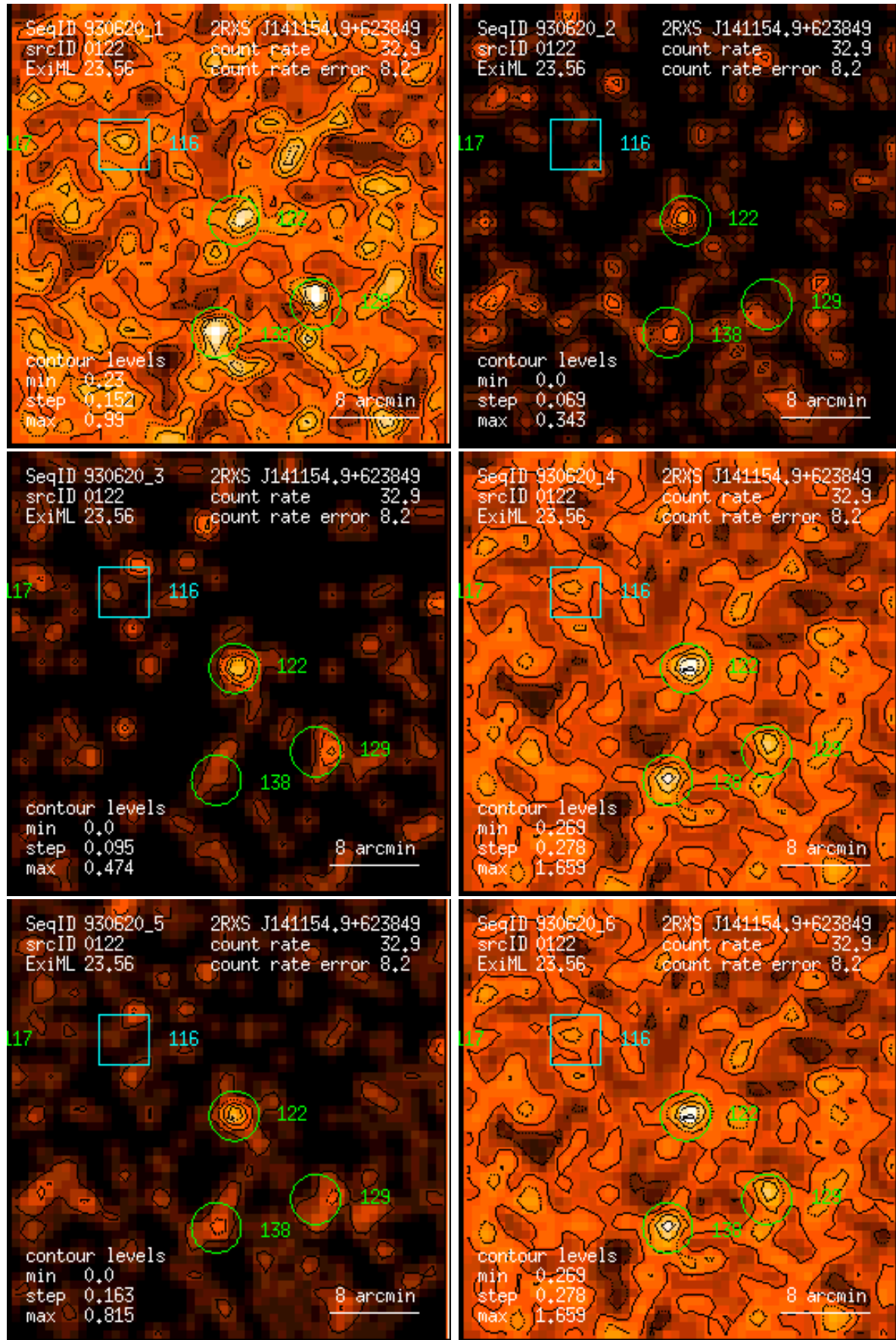
Figure 122: RASS 930620: detection 0122: band rate images, Gaussian filter: (1) PSPC channels 11 – 41, (2) 52 – 90, (3) 91 – 201, (4) 11 – 235, (5) 52 – 201, (6) 11 – 201. Broad band rates in counts/ks. Band rate contour levels in counts/ks/arcmin 2 .
