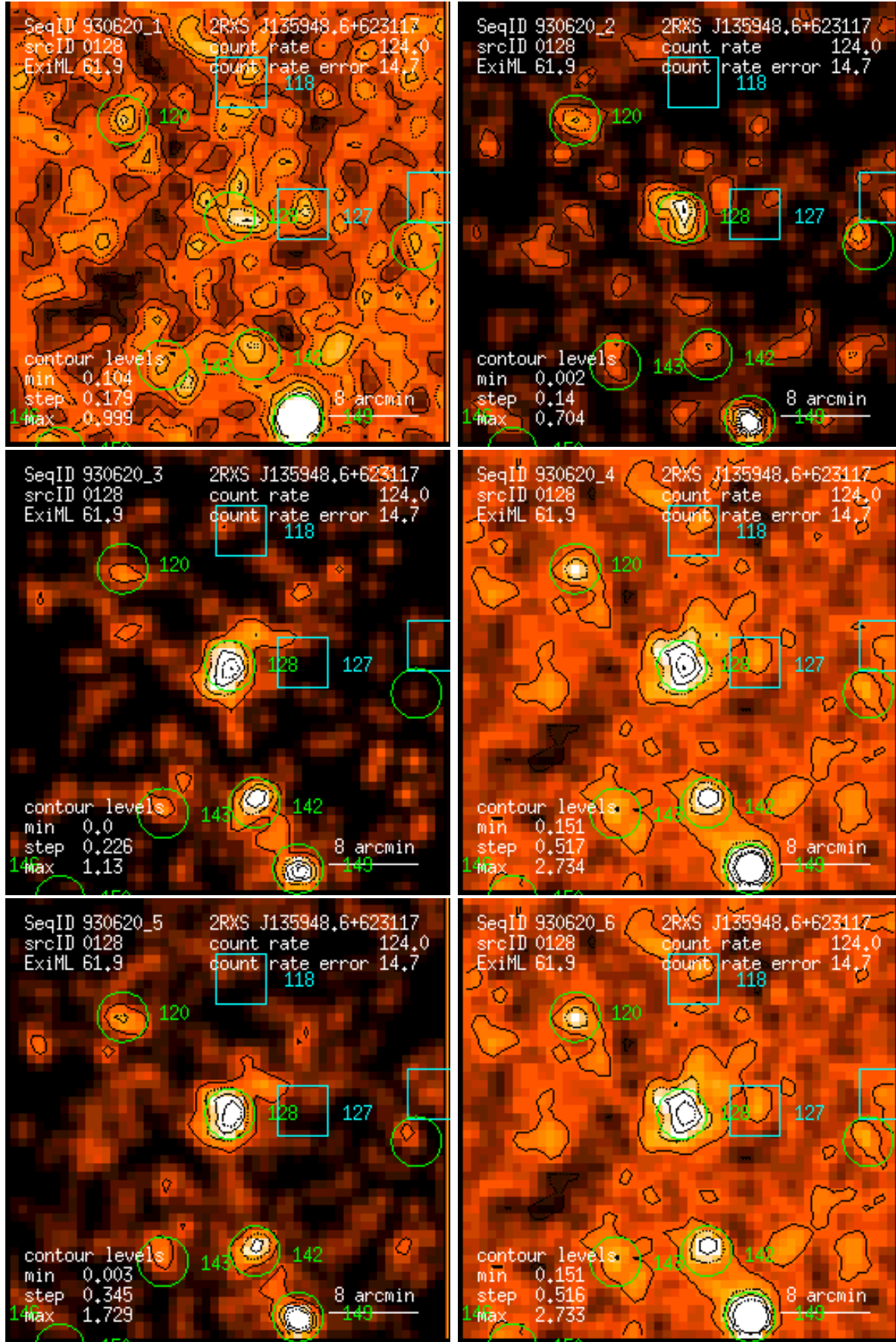
Figure 128: RASS 930620: detection 0128: band rate images, Gaussian filter: (1) PSPC channels 11 – 41, (2) 52 – 90, (3) 91 – 201, (4) 11 – 235, (5) 52 – 201, (6) 11 – 201. Broad band rates in counts/ks. Band rate contour levels in counts/ks/arcmin 2 .
