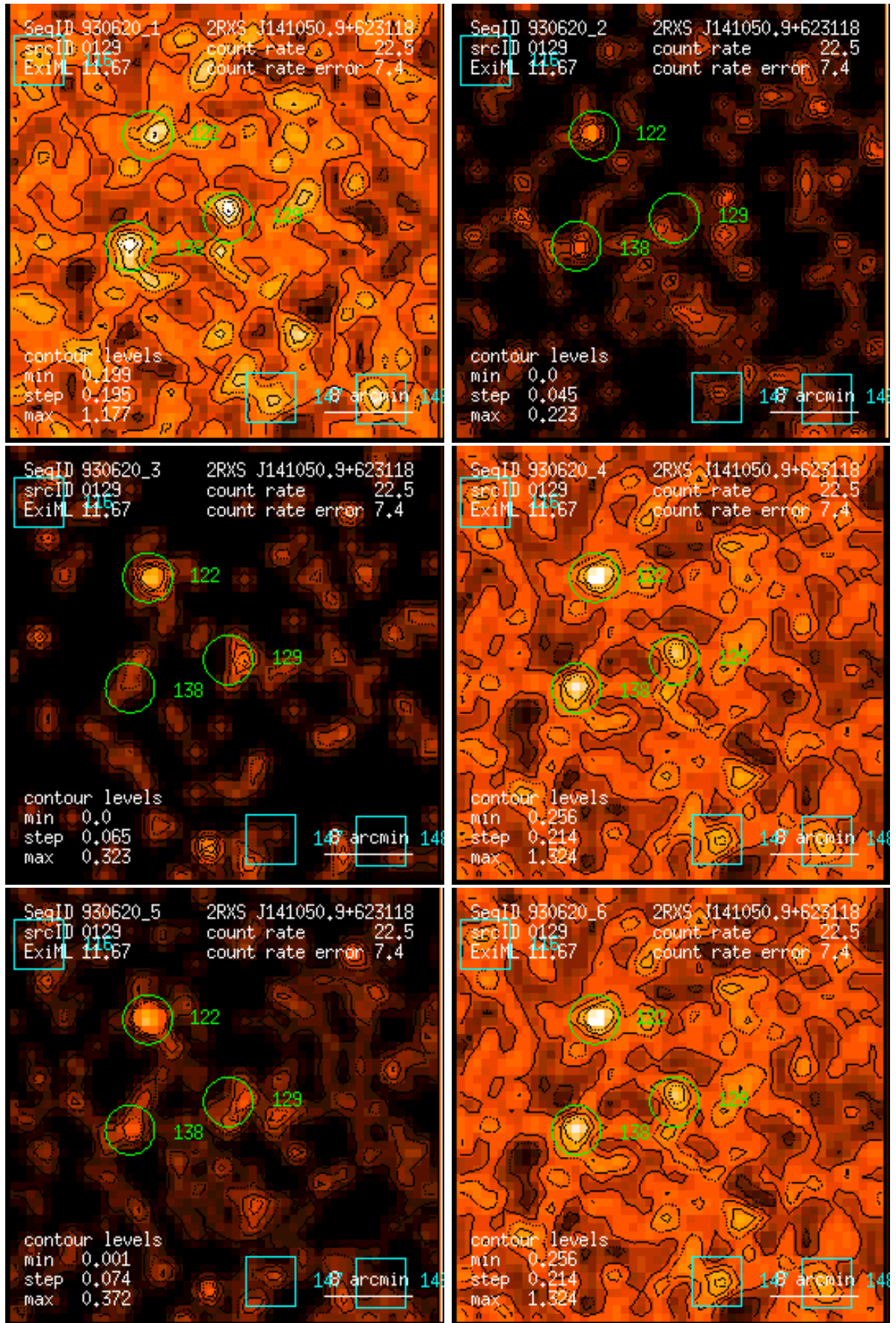
Figure 129: RASS 930620: detection 0129: band rate images, Gaussian filter: (1) PSPC channels 11 – 41, (2) 52 – 90, (3) 91 – 201, (4) 11 – 235, (5) 52 – 201, (6) 11 – 201. Broad band rates in counts/ks. Band rate contour levels in counts/ks/arcmin 2 .
