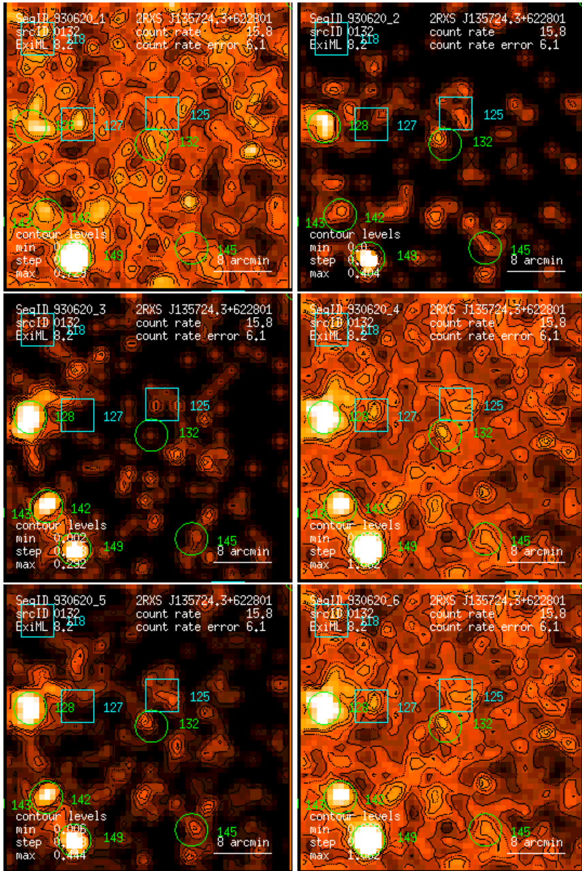
Figure 132: RASS 930620: detection 0132: band rate images, Gaussian filter: (1) PSPC channels 11 – 41, (2) 52 – 90, (3) 91 – 201, (4) 11 – 235, (5) 52 – 201, (6) 11 – 201. Broad band rates in counts/ks. Band rate contour levels in counts/ks/arcmin 2 .
