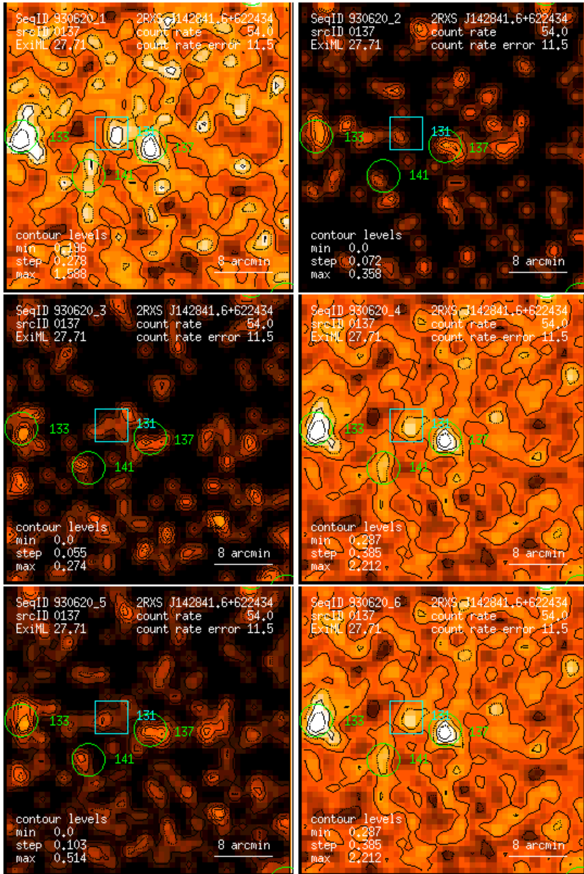
Figure 137: RASS 930620: detection 0137: band rate images, Gaussian filter: (1) PSPC channels 11 – 41, (2) 52 – 90, (3) 91 – 201, (4) 11 – 235, (5) 52 – 201, (6) 11 – 201. Broad band rates in counts/ks. Band rate contour levels in counts/ks/arcmin 2 .
