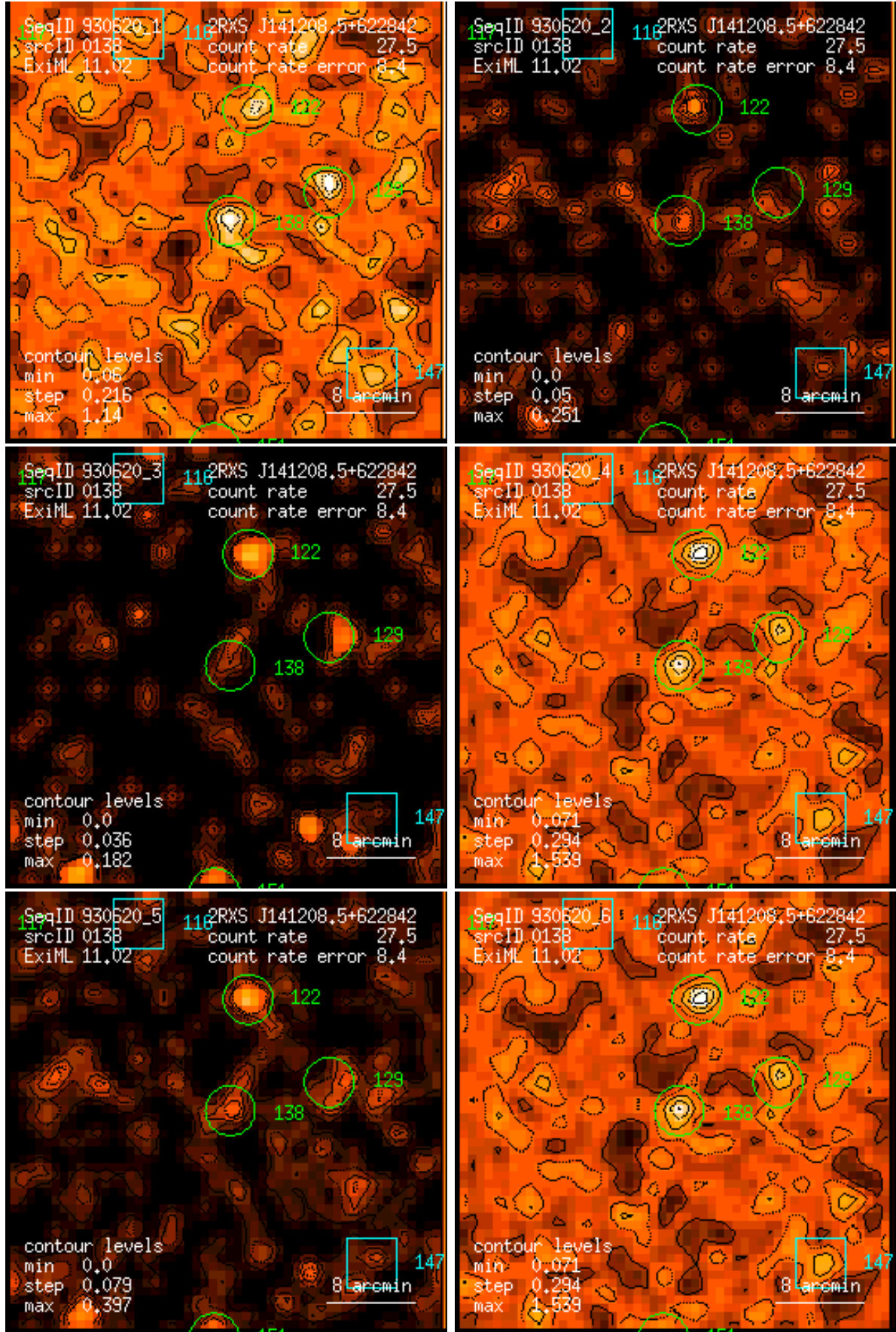
Figure 138: RASS 930620: detection 0138: band rate images, Gaussian filter: (1) PSPC channels 11 – 41, (2) 52 – 90, (3) 91 – 201, (4) 11 – 235, (5) 52 – 201, (6) 11 – 201. Broad band rates in counts/ks. Band rate contour levels in counts/ks/arcmin 2 .
