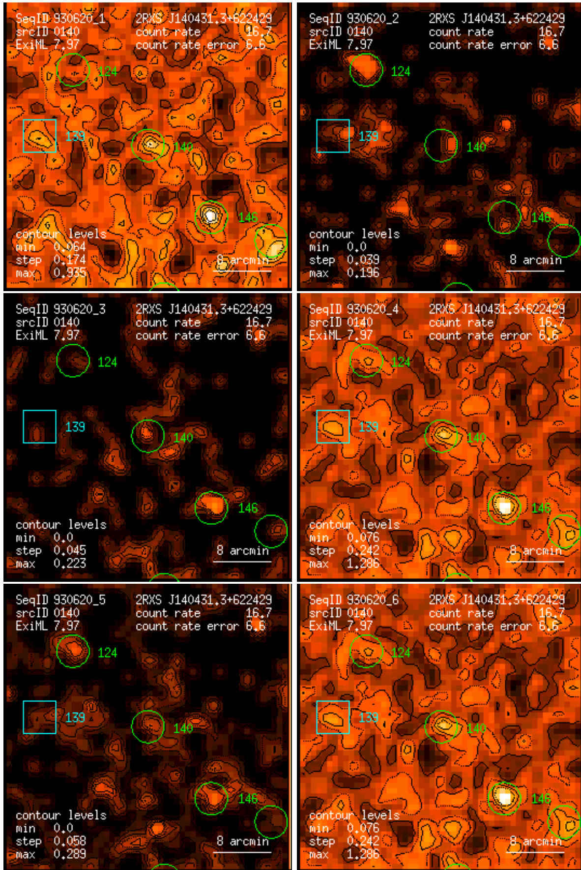
Figure 140: RASS 930620: detection 0140: band rate images, Gaussian filter: (1) PSPC channels 11 – 41, (2) 52 – 90, (3) 91 – 201, (4) 11 – 235, (5) 52 – 201, (6) 11 – 201. Broad band rates in counts/ks. Band rate contour levels in counts/ks/arcmin 2 .
