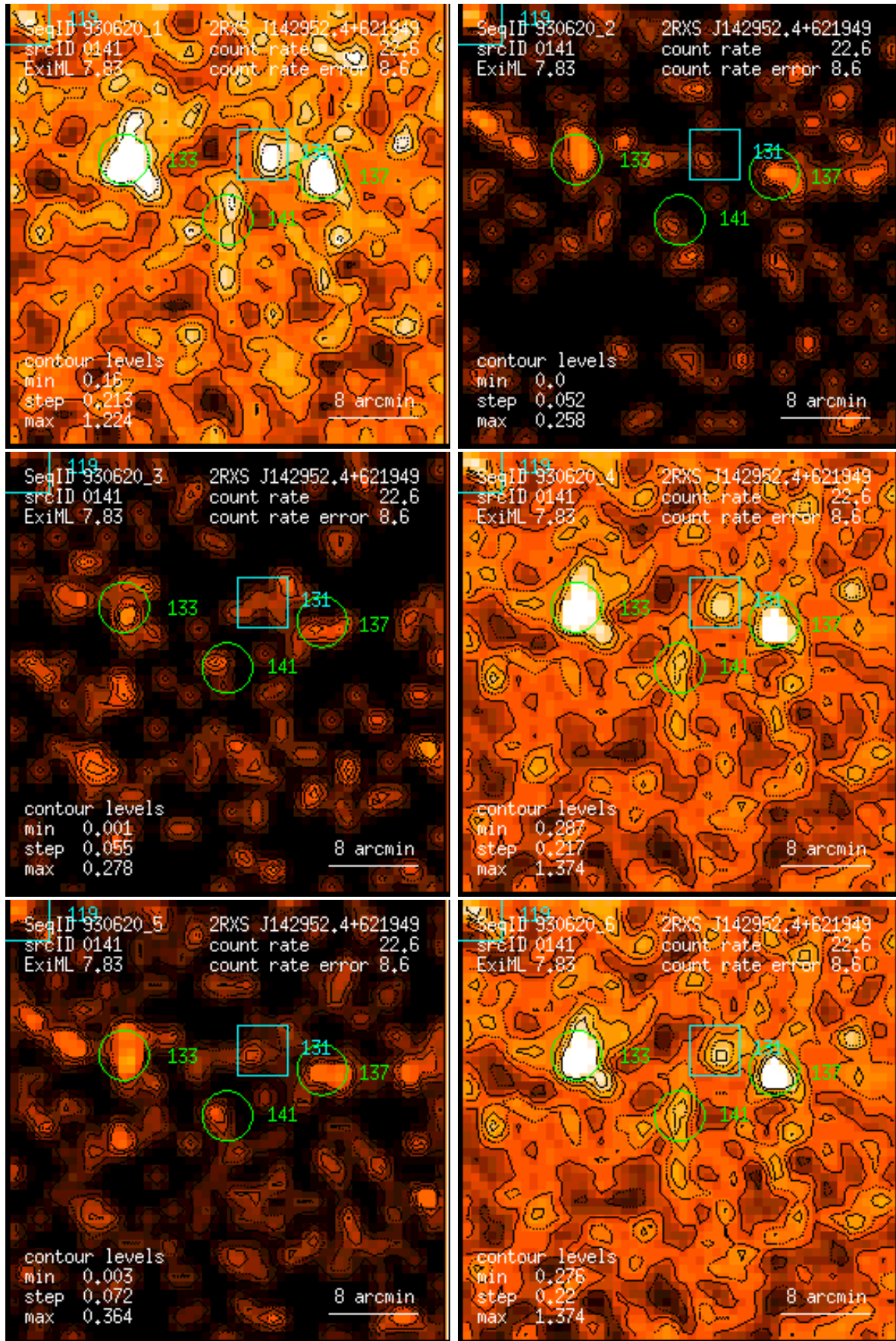
Figure 141: RASS 930620: detection 0141: band rate images, Gaussian filter: (1) PSPC channels 11 – 41, (2) 52 – 90, (3) 91 – 201, (4) 11 – 235, (5) 52 – 201, (6) 11 – 201. Broad band rates in counts/ks. Band rate contour levels in counts/ks/arcmin 2 .
