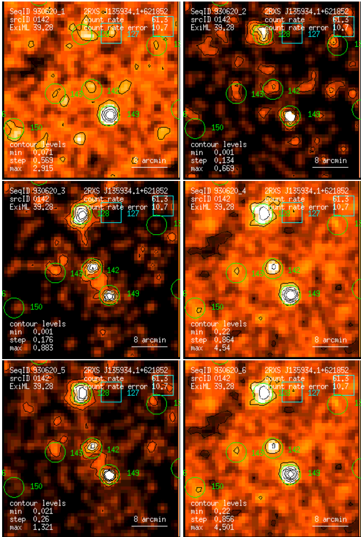
Figure 142: RASS 930620: detection 0142: band rate images, Gaussian filter: (1) PSPC channels 11 – 41, (2) 52 – 90, (3) 91 – 201, (4) 11 – 235, (5) 52 – 201, (6) 11 – 201. Broad band rates in counts/ks. Band rate contour levels in counts/ks/arcmin 2 .
