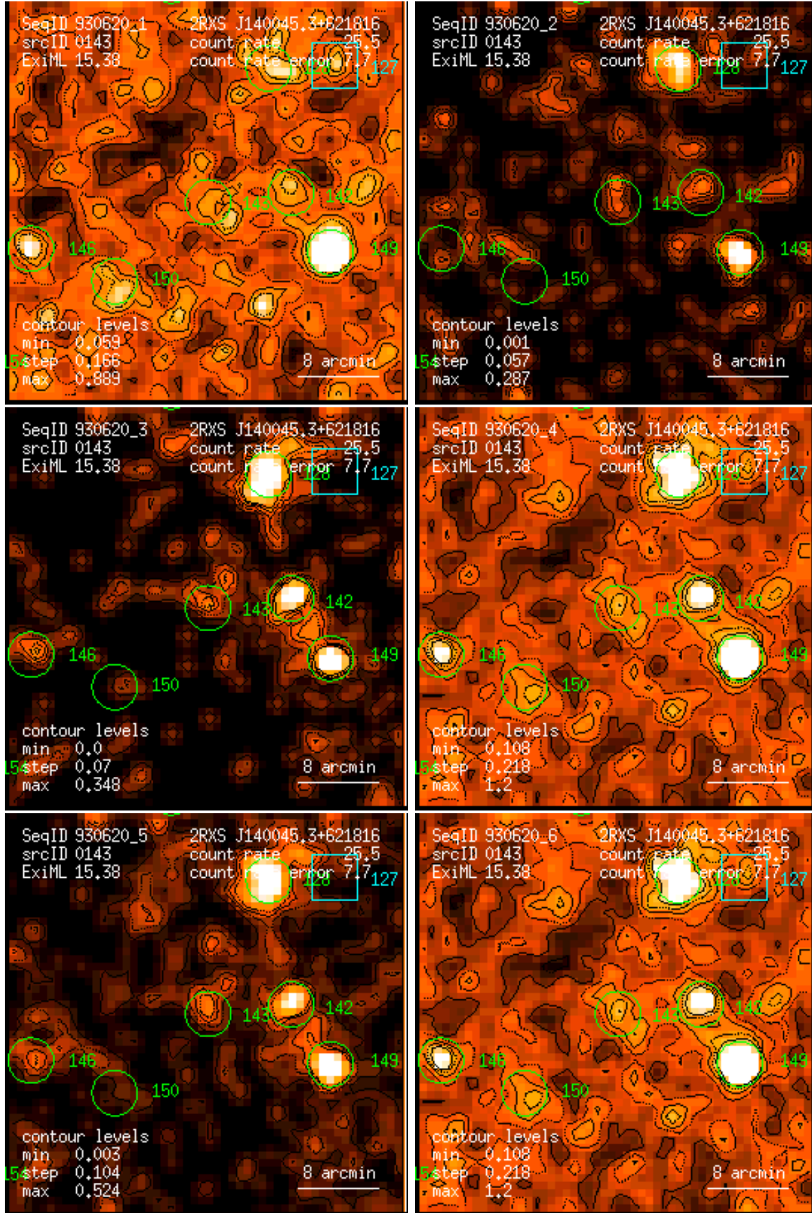
Figure 143: RASS 930620: detection 0143: band rate images, Gaussian filter: (1) PSPC channels 11 – 41, (2) 52 – 90, (3) 91 – 201, (4) 11 – 235, (5) 52 – 201, (6) 11 – 201. Broad band rates in counts/ks. Band rate contour levels in counts/ks/arcmin 2 .
