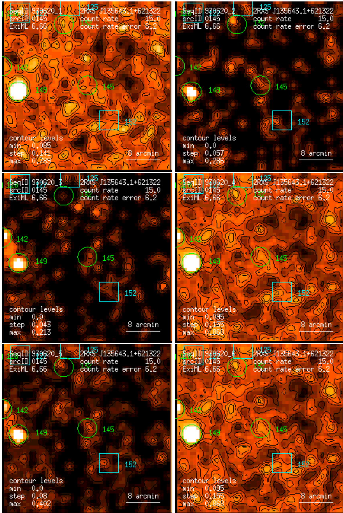
Figure 145: RASS 930620: detection 0145: band rate images, Gaussian filter: (1) PSPC channels 11 – 41, (2) 52 – 90, (3) 91 – 201, (4) 11 – 235, (5) 52 – 201, (6) 11 – 201. Broad band rates in counts/ks. Band rate contour levels in counts/ks/arcmin 2 .
