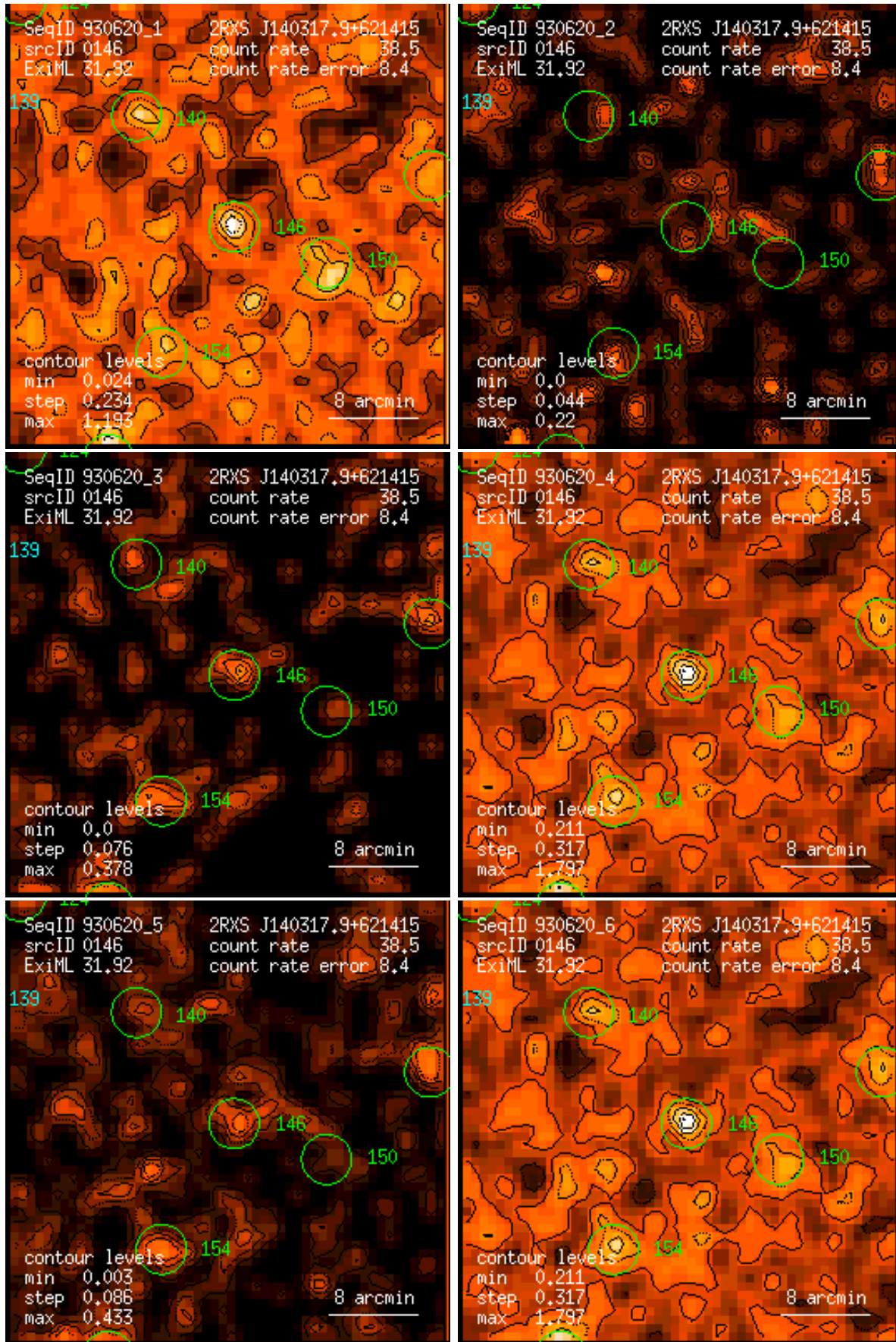
Figure 146: RASS 930620: detection 0146: band rate images, Gaussian filter: (1) PSPC channels 11 – 41, (2) 52 – 90, (3) 91 – 201, (4) 11 – 235, (5) 52 – 201, (6) 11 – 201. Broad band rates in counts/ks. Band rate contour levels in counts/ks/arcmin 2 .
