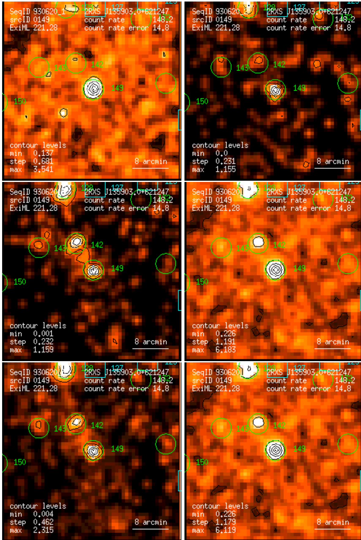
Figure 149: RASS 930620: detection 0149: band rate images, Gaussian filter: (1) PSPC channels 11 – 41, (2) 52 – 90, (3) 91 – 201, (4) 11 – 235, (5) 52 – 201, (6) 11 – 201. Broad band rates in counts/ks. Band rate contour levels in counts/ks/arcmin 2 .
