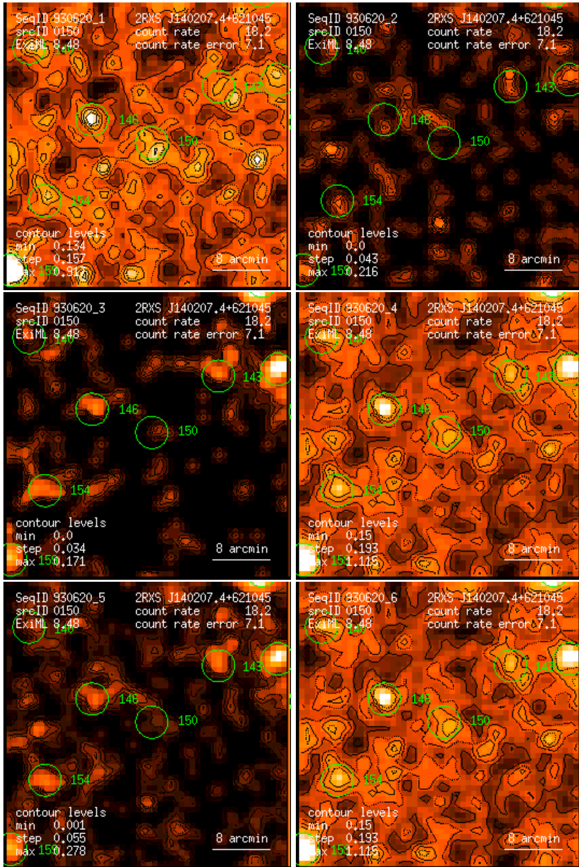
Figure 150: RASS 930620: detection 0150: band rate images, Gaussian filter: (1) PSPC channels 11 – 41, (2) 52 – 90, (3) 91 – 201, (4) 11 – 235, (5) 52 – 201, (6) 11 – 201. Broad band rates in counts/ks. Band rate contour levels in counts/ks/arcmin 2 .
