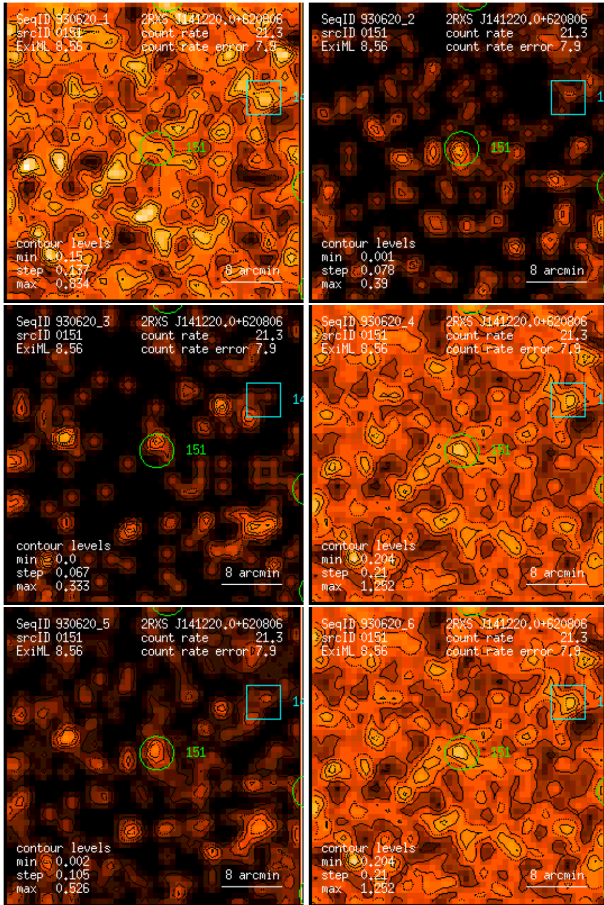
Figure 151: RASS 930620: detection 0151: band rate images, Gaussian filter: (1) PSPC channels 11 – 41, (2) 52 – 90, (3) 91 – 201, (4) 11 – 235, (5) 52 – 201, (6) 11 – 201. Broad band rates in counts/ks. Band rate contour levels in counts/ks/arcmin 2 .
