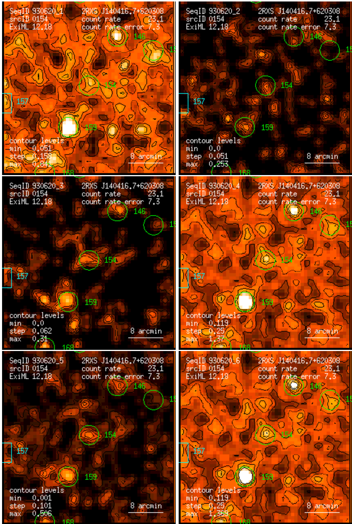
Figure 154: RASS 930620: detection 0154: band rate images, Gaussian filter: (1) PSPC channels 11 – 41, (2) 52 – 90, (3) 91 – 201, (4) 11 – 235, (5) 52 – 201, (6) 11 – 201. Broad band rates in counts/ks. Band rate contour levels in counts/ks/arcmin 2 .
