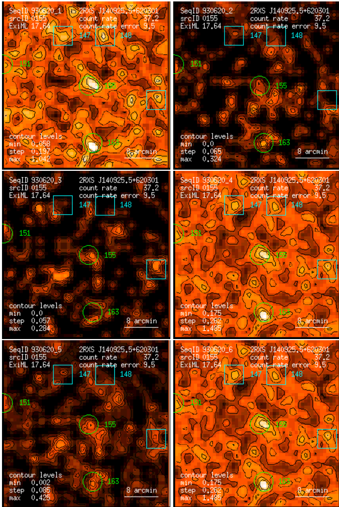
Figure 155: RASS 930620: detection 0155: band rate images, Gaussian filter: (1) PSPC channels 11 – 41, (2) 52 – 90, (3) 91 – 201, (4) 11 – 235, (5) 52 – 201, (6) 11 – 201. Broad band rates in counts/ks. Band rate contour levels in counts/ks/arcmin 2 .
