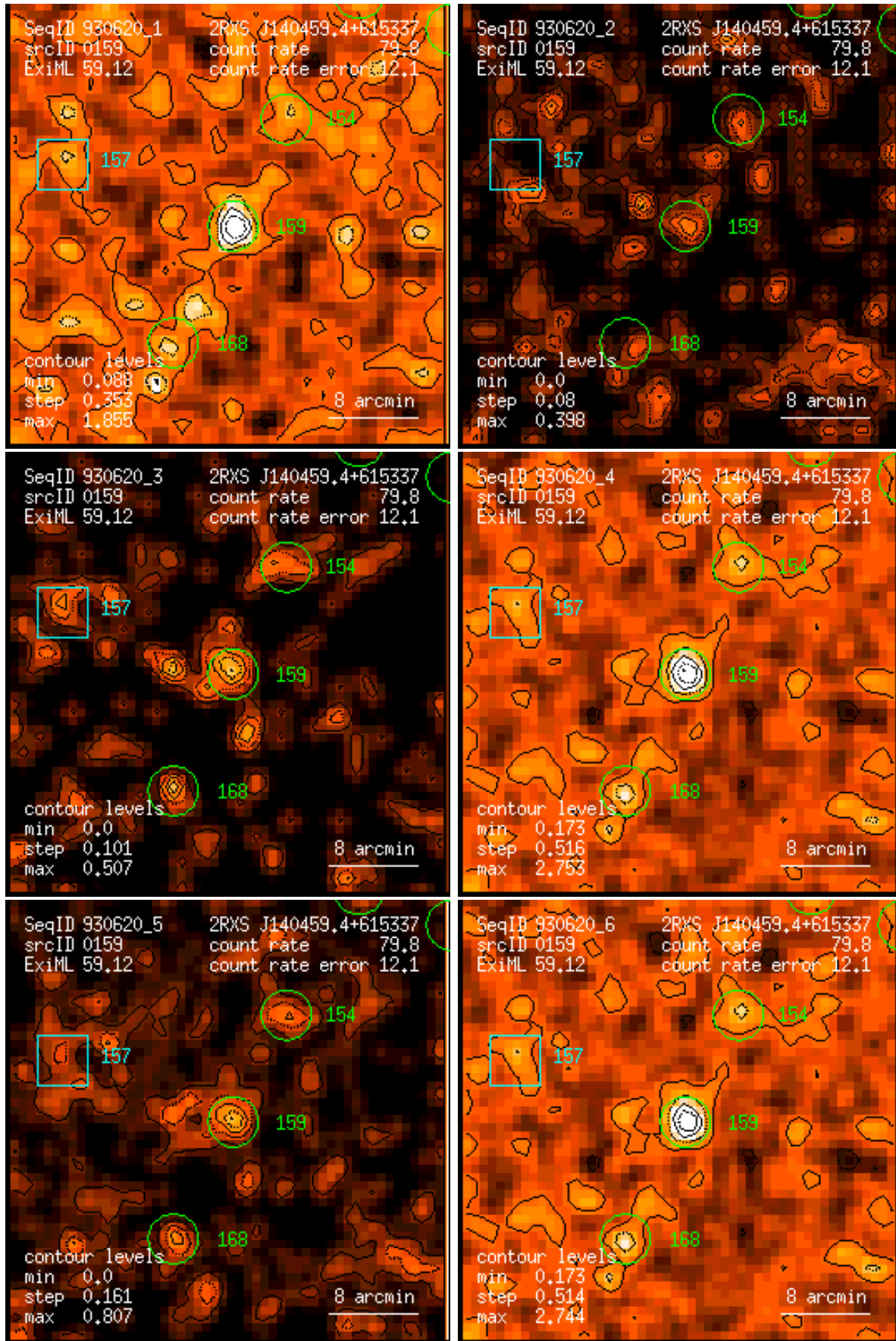
Figure 159: RASS 930620: detection 0159: band rate images, Gaussian filter: (1) PSPC channels 11 – 41, (2) 52 – 90, (3) 91 – 201, (4) 11 – 235, (5) 52 – 201, (6) 11 – 201. Broad band rates in counts/ks. Band rate contour levels in counts/ks/arcmin 2 .
