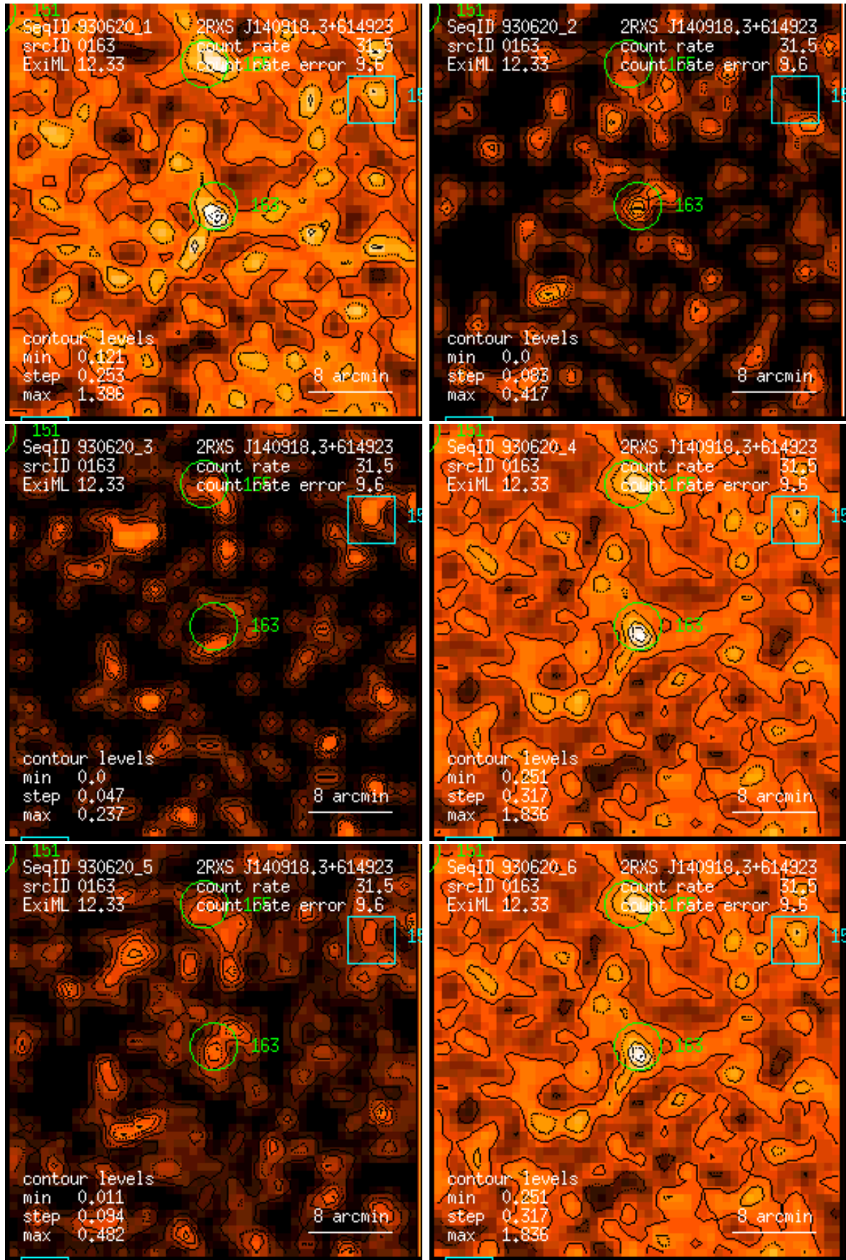
Figure 163: RASS 930620: detection 0163: band rate images, Gaussian filter: (1) PSPC channels 11 – 41, (2) 52 – 90, (3) 91 – 201, (4) 11 – 235, (5) 52 – 201, (6) 11 – 201. Broad band rates in counts/ks. Band rate contour levels in counts/ks/arcmin 2 .
