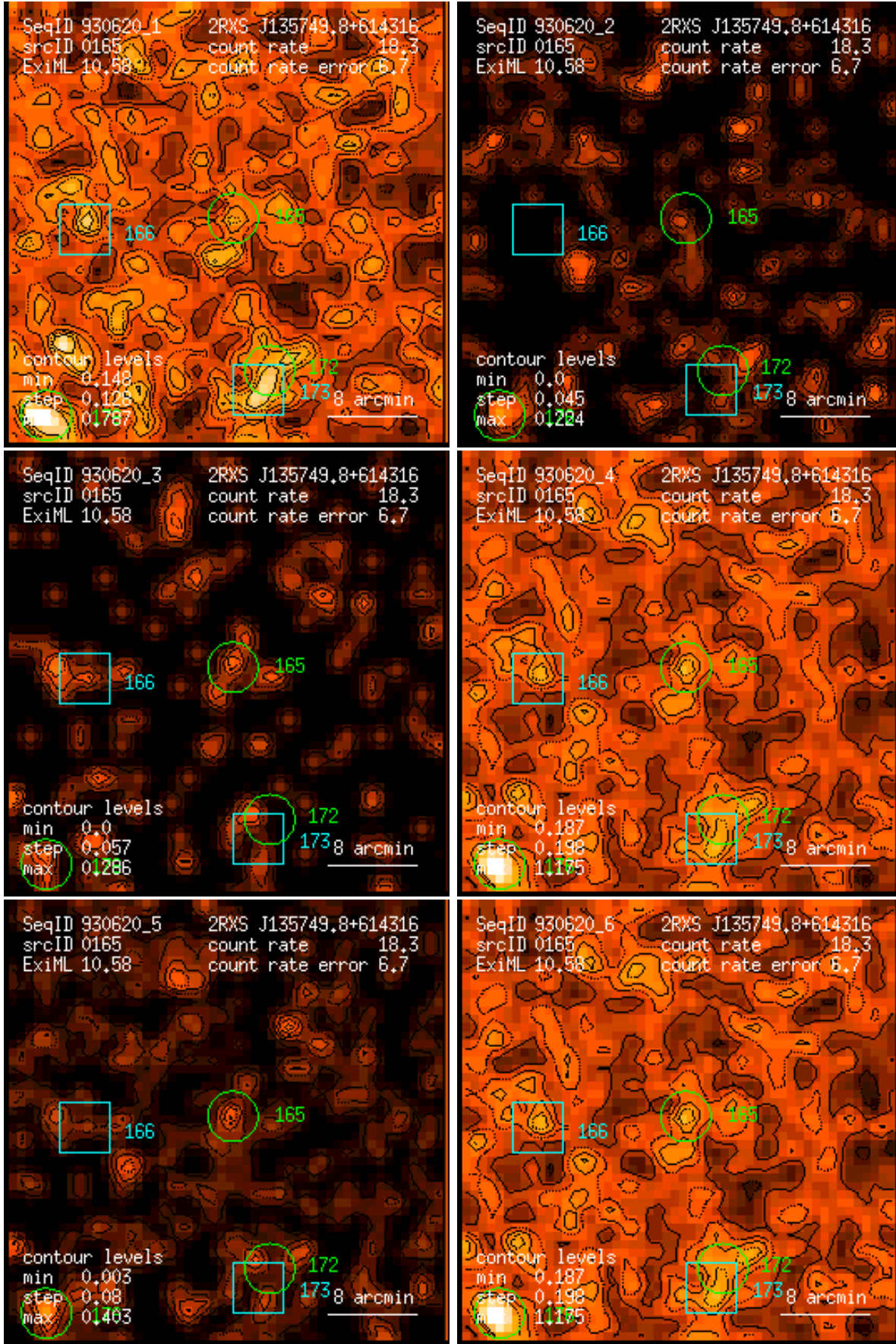
Figure 165: RASS 930620: detection 0165: band rate images, Gaussian filter: (1) PSPC channels 11 – 41, (2) 52 – 90, (3) 91 – 201, (4) 11 – 235, (5) 52 – 201, (6) 11 – 201. Broad band rates in counts/ks. Band rate contour levels in counts/ks/arcmin 2 .
