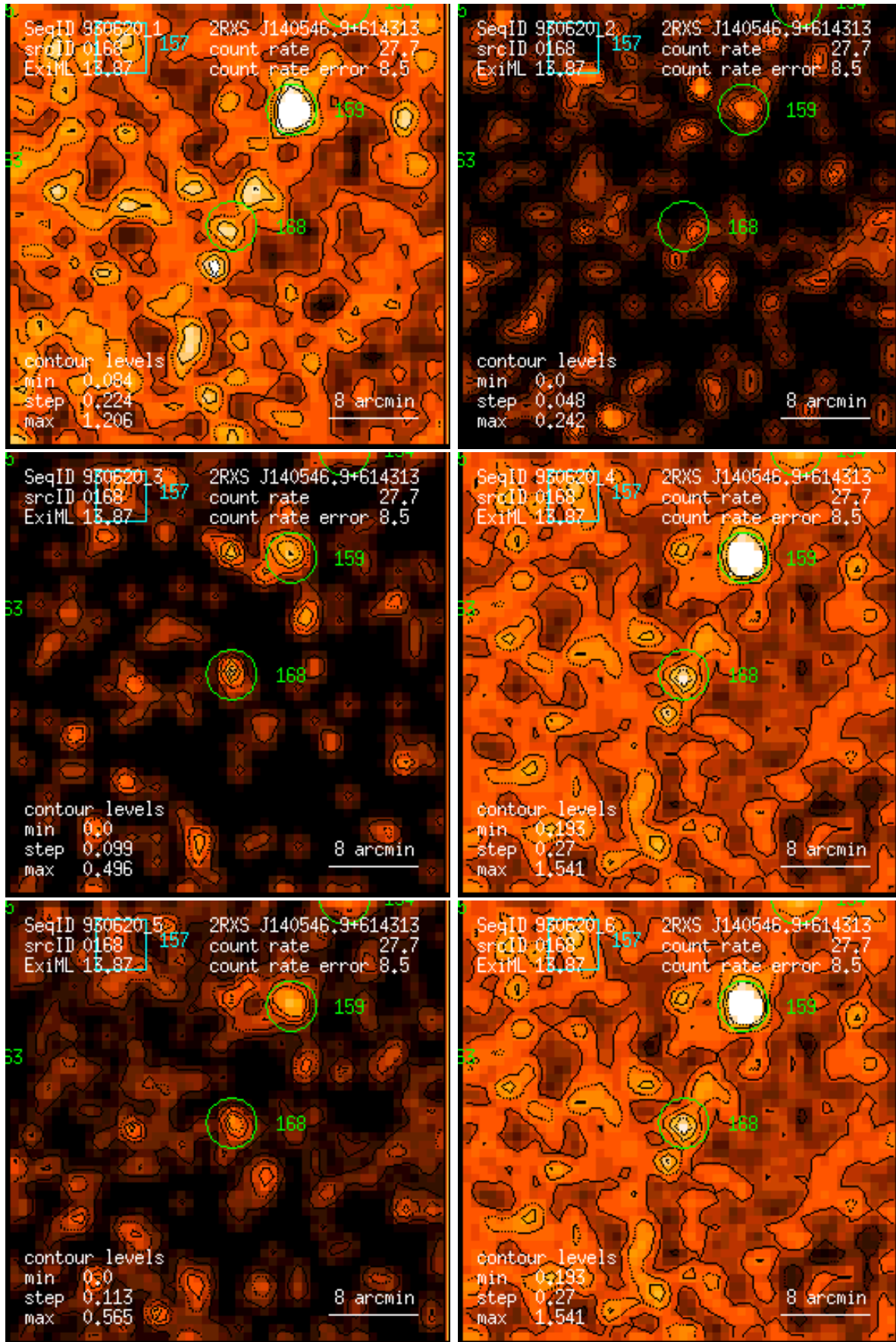
Figure 168: RASS 930620: detection 0168: band rate images, Gaussian filter: (1) PSPC channels 11 – 41, (2) 52 – 90, (3) 91 – 201, (4) 11 – 235, (5) 52 – 201, (6) 11 – 201. Broad band rates in counts/ks. Band rate contour levels in counts/ks/arcmin 2 .
