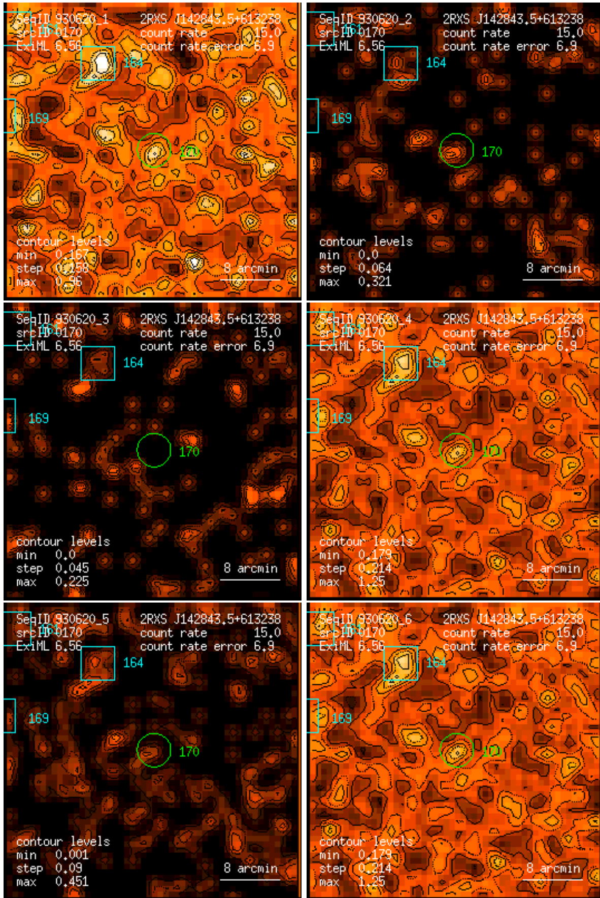
Figure 170: RASS 930620: detection 0170: band rate images, Gaussian filter: (1) PSPC channels 11 – 41, (2) 52 – 90, (3) 91 – 201, (4) 11 – 235, (5) 52 – 201, (6) 11 – 201. Broad band rates in counts/ks. Band rate contour levels in counts/ks/arcmin 2 .
