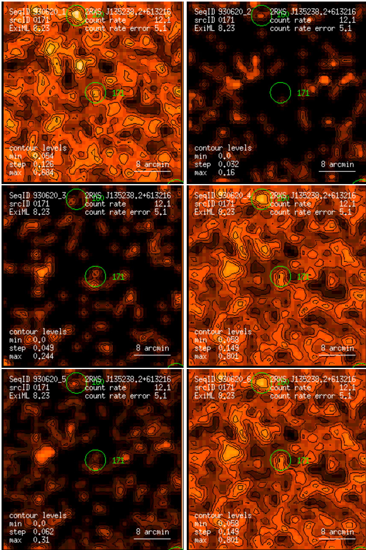
Figure 171: RASS 930620: detection 0171: band rate images, Gaussian filter: (1) PSPC channels 11 – 41, (2) 52 – 90, (3) 91 – 201, (4) 11 – 235, (5) 52 – 201, (6) 11 – 201. Broad band rates in counts/ks. Band rate contour levels in counts/ks/arcmin 2 .
