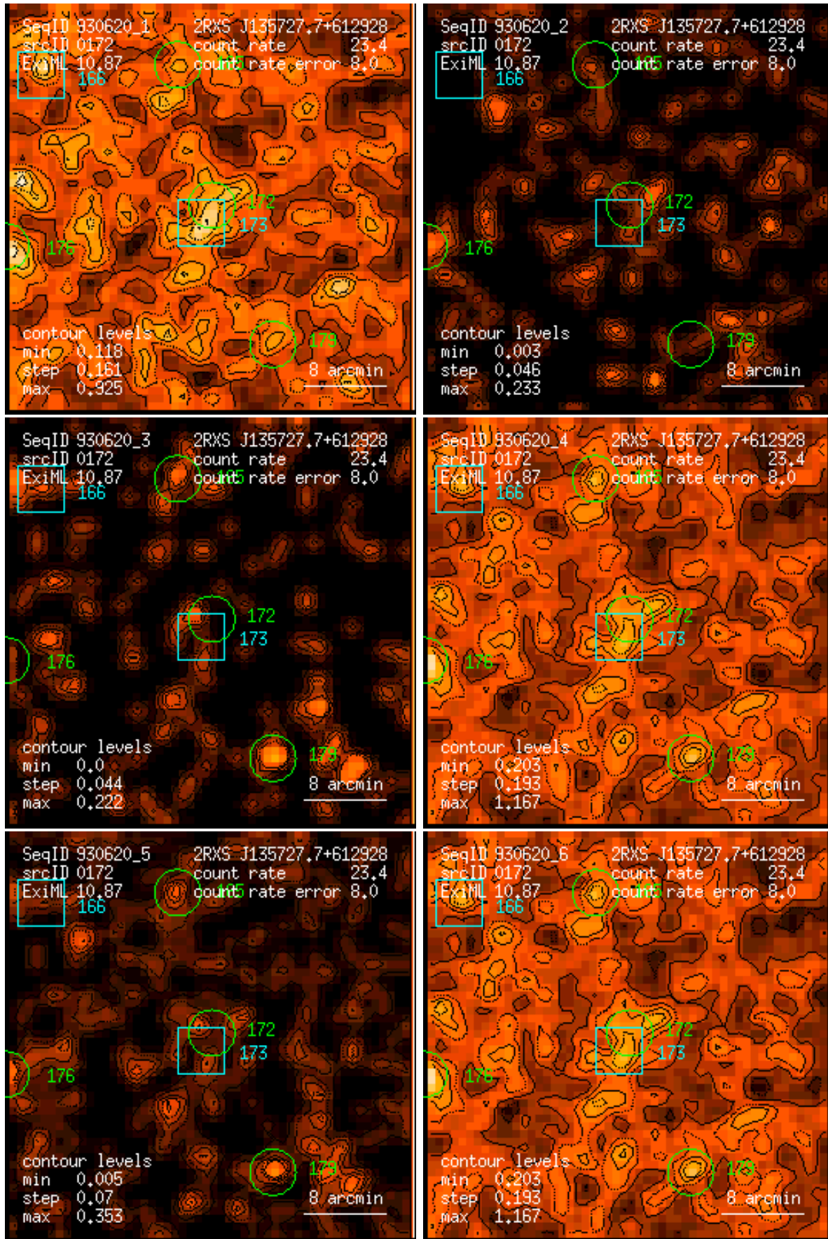
Figure 172: RASS 930620: detection 0172: band rate images, Gaussian filter: (1) PSPC channels 11 – 41, (2) 52 – 90, (3) 91 – 201, (4) 11 – 235, (5) 52 – 201, (6) 11 – 201. Broad band rates in counts/ks. Band rate contour levels in counts/ks/arcmin 2 .
